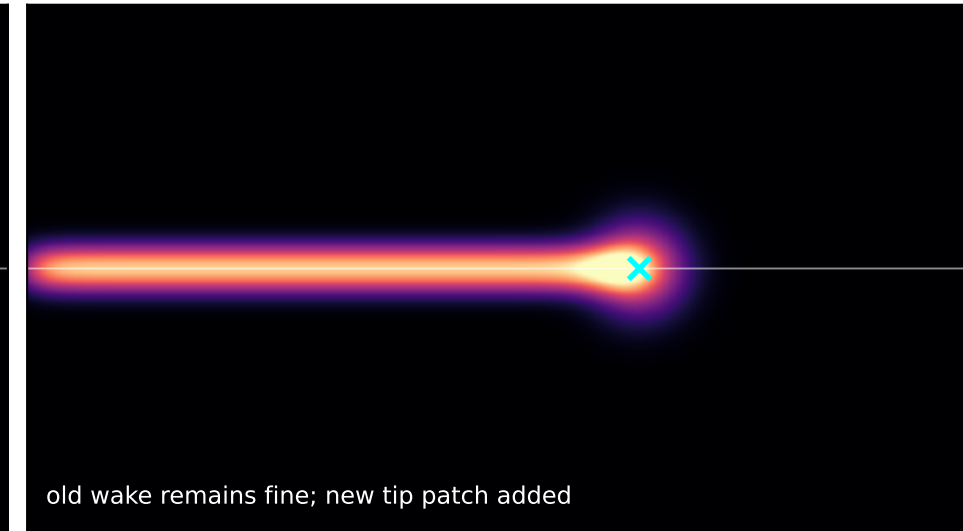
v4 add-only refinement phase field alpha
