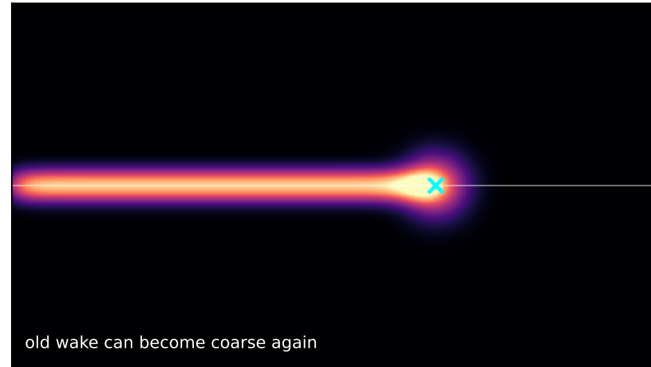
S2 non-nested remesh phase field alpha
