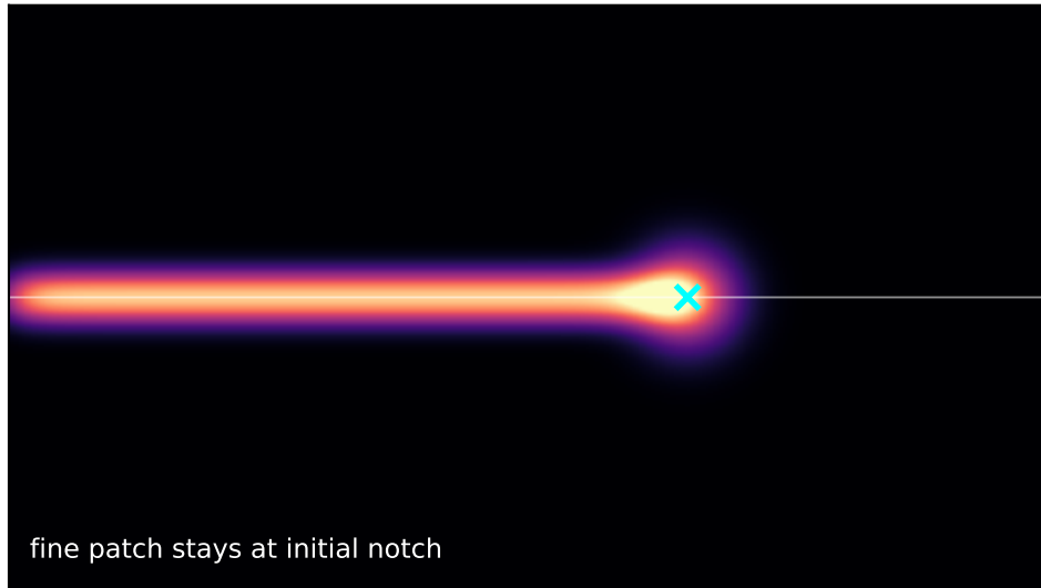
S1 static refine phase field alpha
