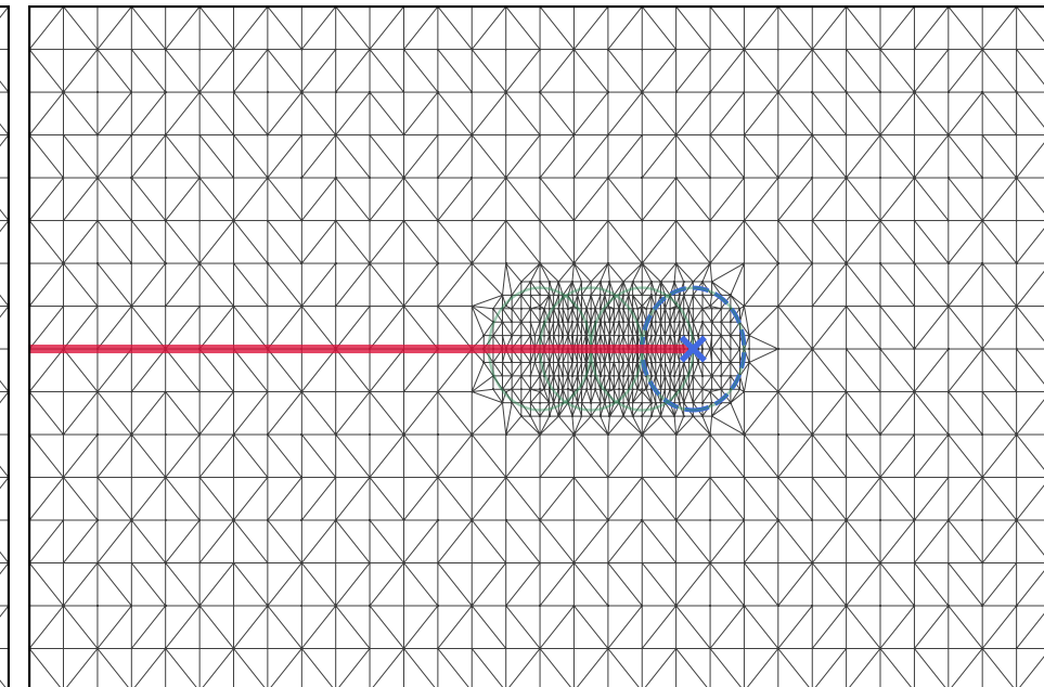
mesh / quadrature density
