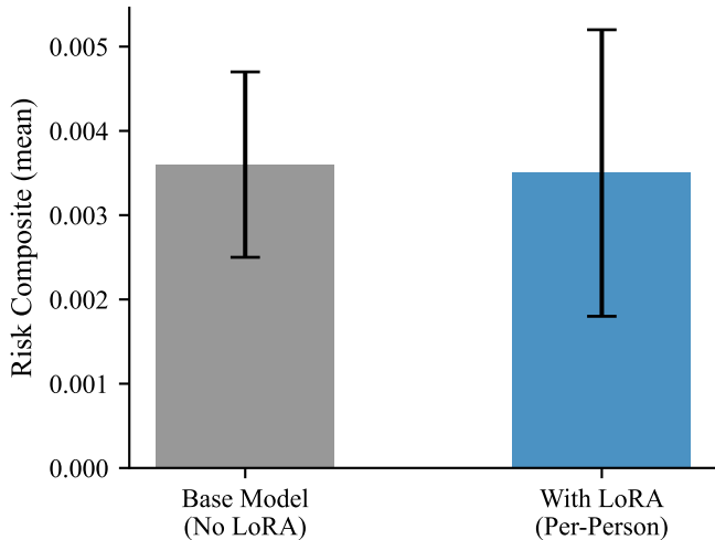
(a) Mean Level
