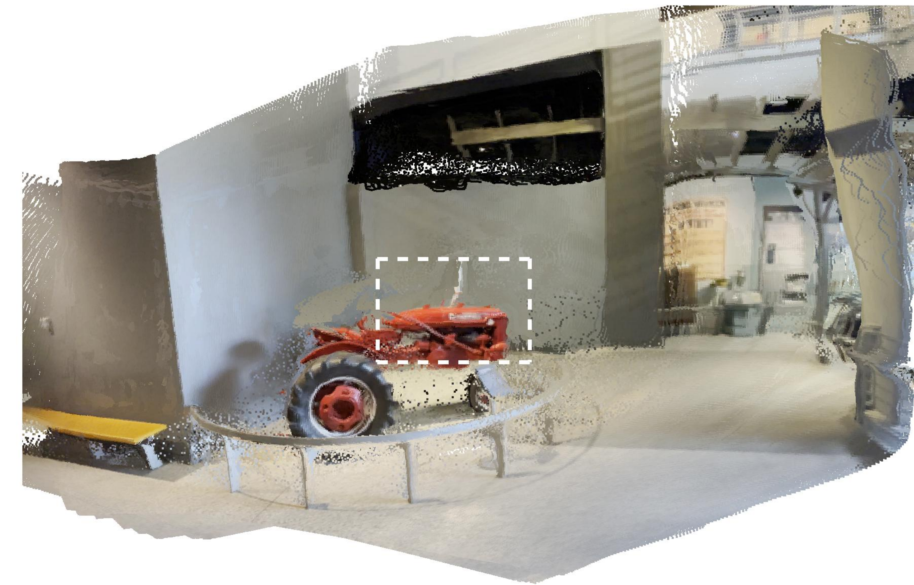
Ground Truth
