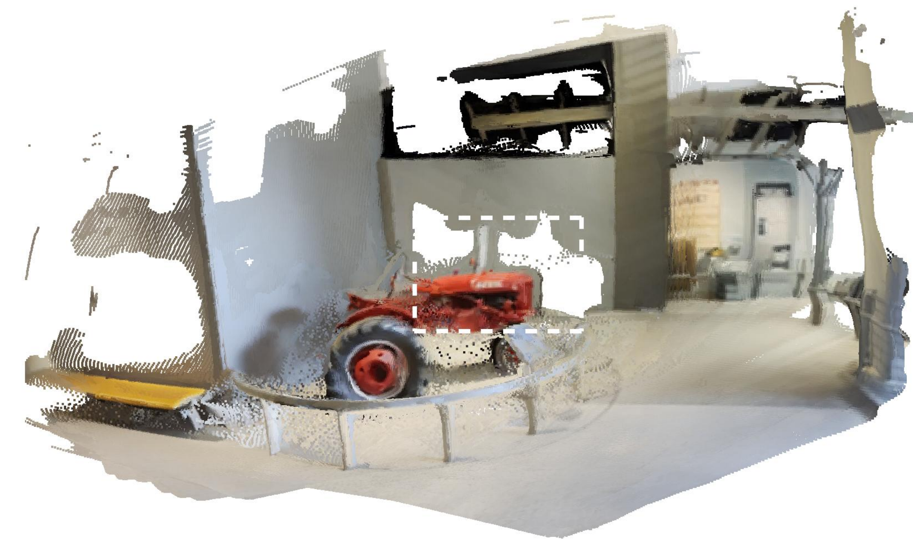
ViewCrafter
