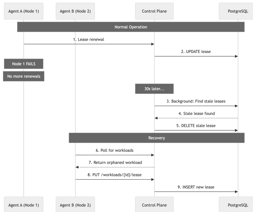
Fig. 4.7. Sequence diagram illustrating fault tolerance through lease expiration. When Agent A fails, the background task expires the stale lease after 30 seconds, enabling Agent B to acquire and reschedule the workload.
