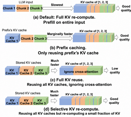
Figure 1: Comparison of different KV cache reuse strategies. Adapted from Jiayi Yao (2025).
