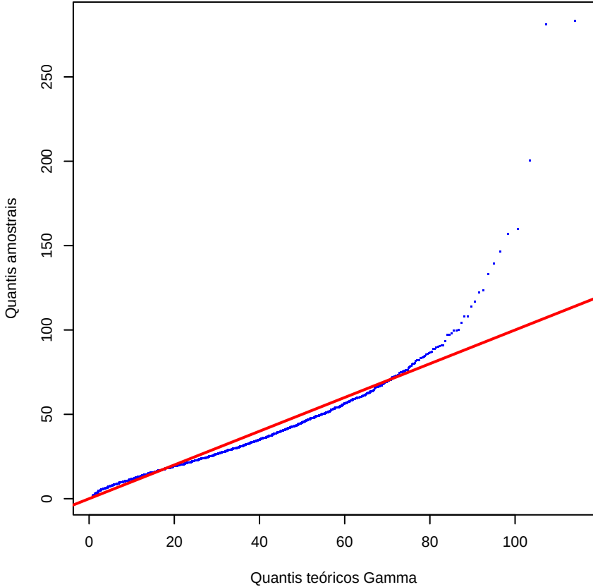
QQ-plot: Consumo vs Gamma
