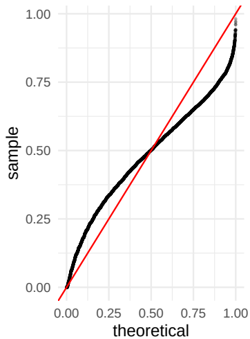
QQ Unif — X
