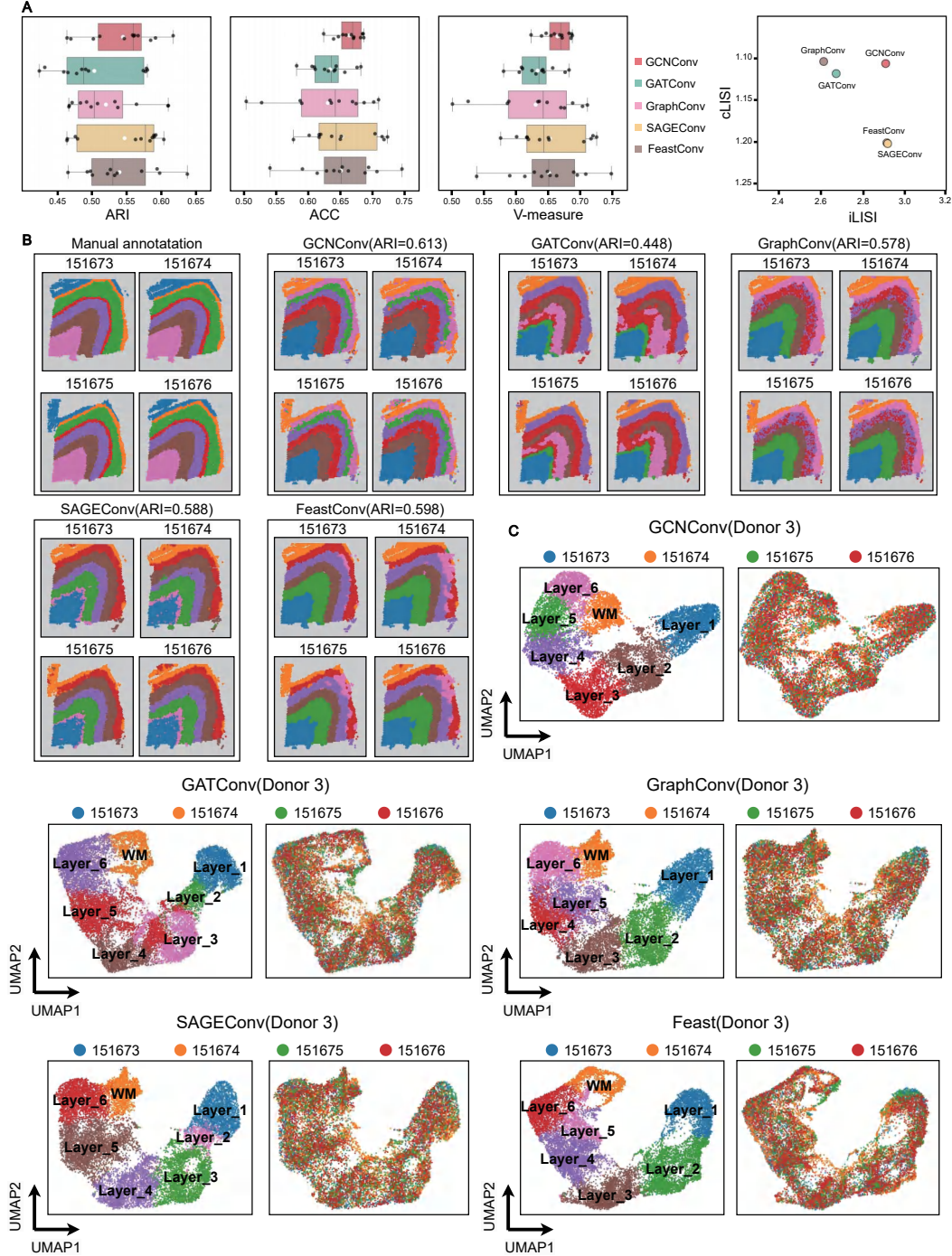
Fig. S17 The impact of applying different graph convolution layers in the backbone network on performance. (A) Bar plots of clustering performance in terms of ARI, ACC, and V-measure scores by applying different graph convolution layers to the SpaBatch backbone network on the DLPFC dataset. The plots also show the iLISI and cLISI scores computed on this dataset. (B) Integration results of four slices from sample 3 of the DLPFC dataset by different graph convolution layers, with identification of spatial domains. (C) UMAP visualizations of the embeddings for Donor 3 (slices 151673|151676) under different graph convolution layers, colored by the identified domains (left) and by batch (right).
