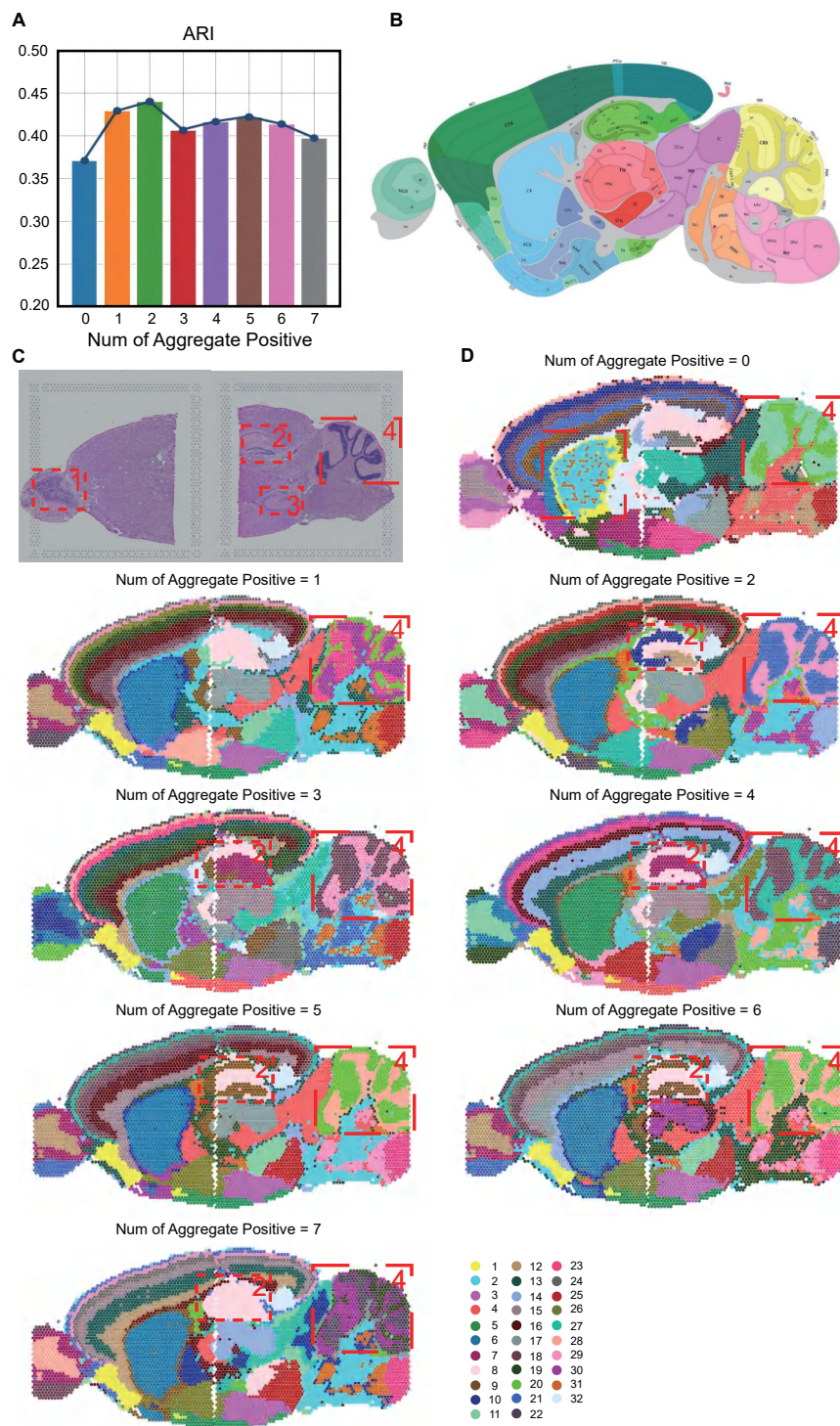
Fig. S19 The impact of the number of positive samples in the Readout triplet aggregation strategy on performance. (A) The bar plot compares the changes in the clustering metric ARI under different numbers of positive samples, while the line plot represents the overall trend. (B) Manual annotation of the sagittal anterior mouse brain (Section 1), from the Allen Mouse Brain Reference Atlas. (C) H&E images of sagittal anterior and posterior sections of Section 1, and the corresponding specific spatial subdomains. (D) Spatial domain identification results on the sagittal anterior mouse brain dataset under different number of positive samples.
