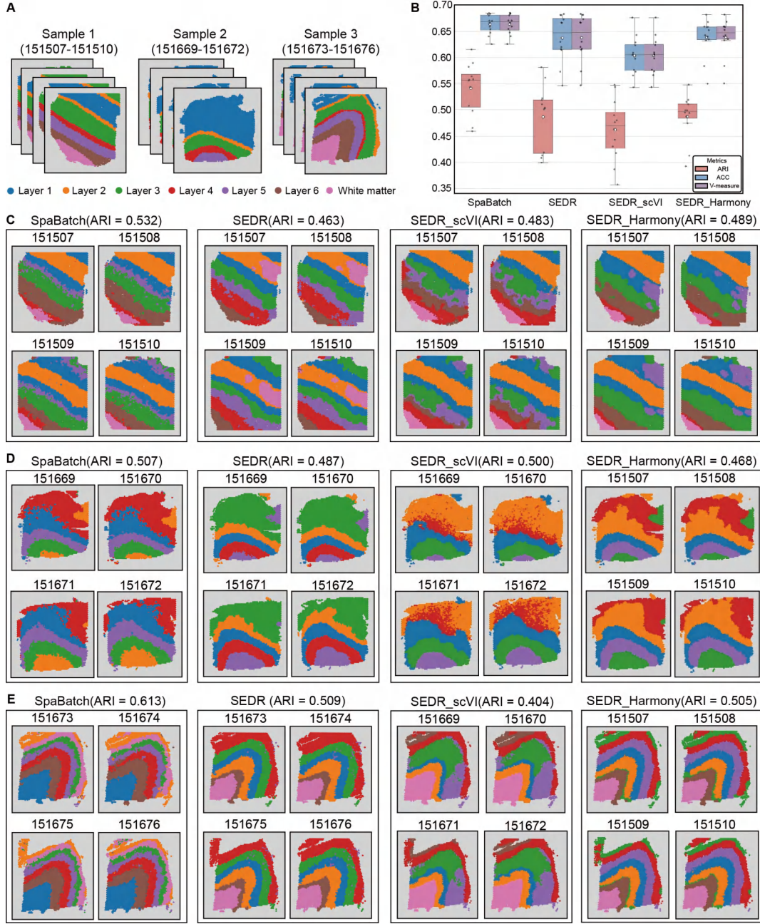
Fig. S20 Performance comparison on the DLPFC dataset with batch correction using scVI and Harmony, followed by graph neural network training. SEDR_scVI and SEDR_Harmony denote batch correction performed first using scVI and Harmony, respectively, followed by training with the graph neural network SEDR. (A) . Three samples of the DLPFC dataset and their manual annotations. (B) . Box plots compare the clustering performance of SpaBatch, SEDR, SEDR_scVI, and SEDR_Harmony on the DLPFC dataset across three metrics. (C) . Spatial domain identification results on the DLPFC dataset sample 1. (D) . Spatial domain identification results on the DLPFC dataset sample 2. (E) . Spatial domain identification results on the DLPFC dataset sample 3.
