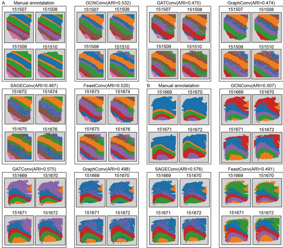
Fig. S18 Integration results of four slices from (A) . Donor 1 and (B) . Donor 2 of the DLPFC dataset by different graph convolution layers, with identification of spatial domains.
