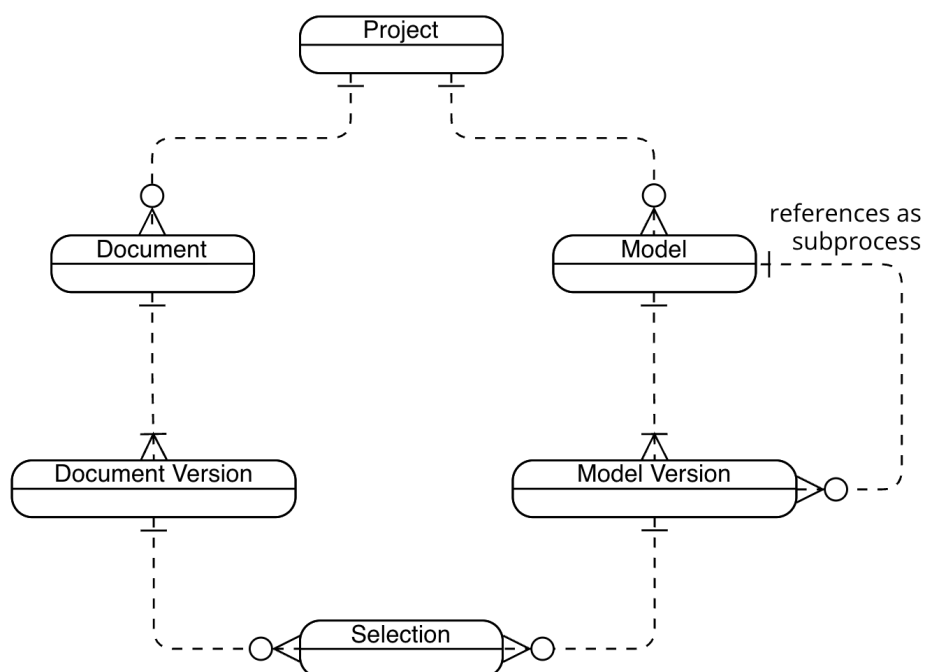
Figure 3 Conceptual data model
