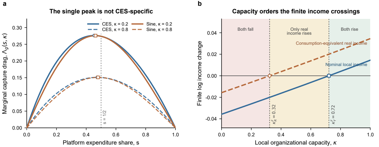
Figure 1: Capture drag and finite capacity thresholds. (a) CES g(s) = 3s(1 - s) and non-CES g(s) = 0.75\sin(\pi s) are shown at \kappa = 0.2 and 0.8 ; both have a unique pre-half peak, and capacity moves it right while lowering it. (b) Finite log-income changes cross zero at \kappa_R^F = 0.32 < \kappa_Y^F = 0.72 . Panel (b) uses the CES specialization with \alpha = 0.35 , \beta = 0.25 , a = 0.4 , \eta = 4 , \varepsilon = 0.08 , \rho_A = 0.8 , (\underline{\rho}_P, \bar{\rho}_P) = (0.1, 0.6) , and (z_0, z_1) = (-0.75, -0.30) . Illustration, not calibration.
