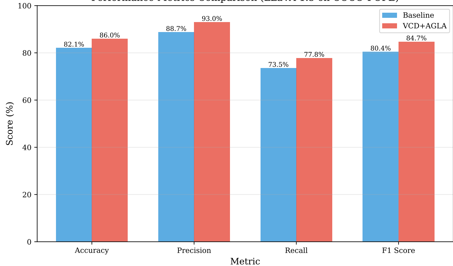
Performance Metrics Comparison (LLaVA-1.5 on COCO-POPE)
