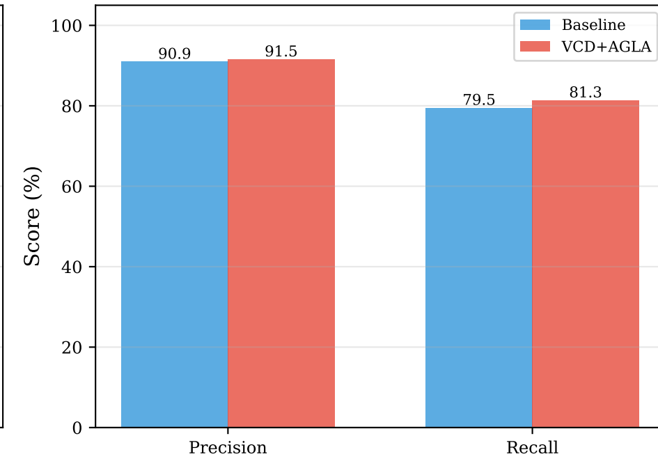
Qwen-VL AOKVQA-POPE
