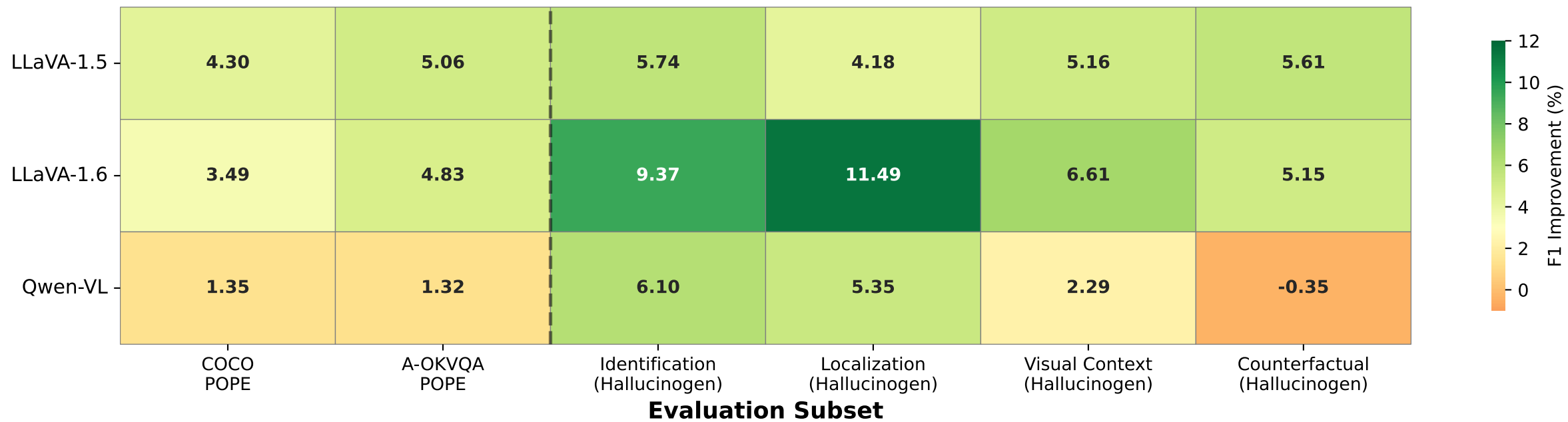
F1 Score Improvements Across All Evaluation Subsets
