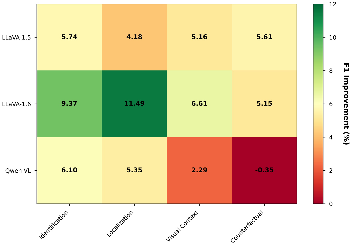
F1 Score Improvements on Hallucinogen Benchmark (VCD+AGLA vs Baseline)
