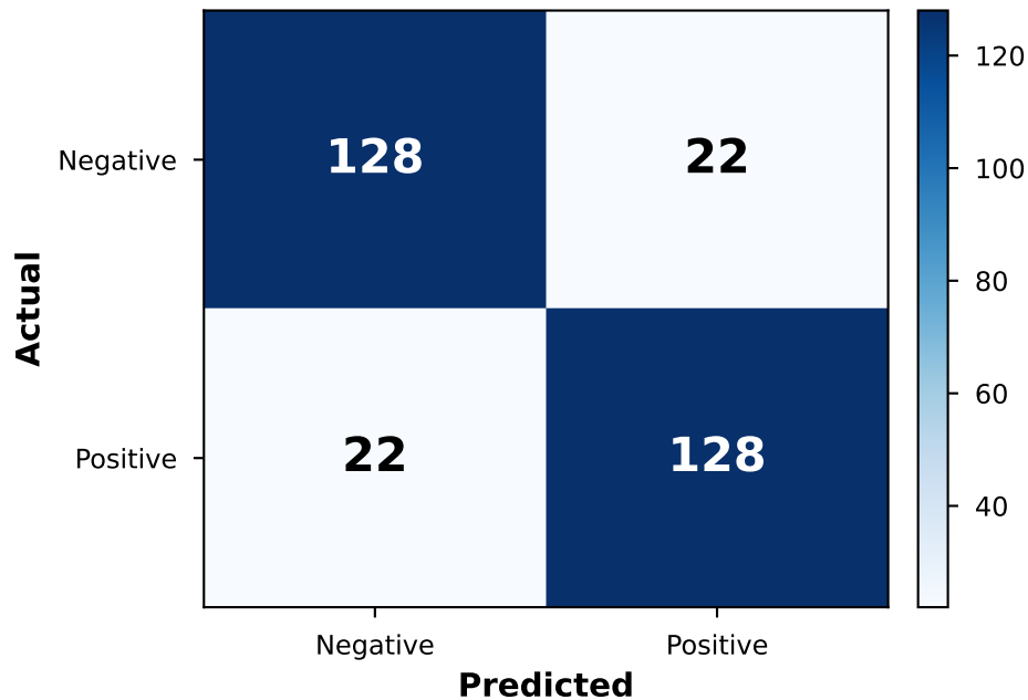
VCD+AGLA (LLaVA-1.5, Identification)
