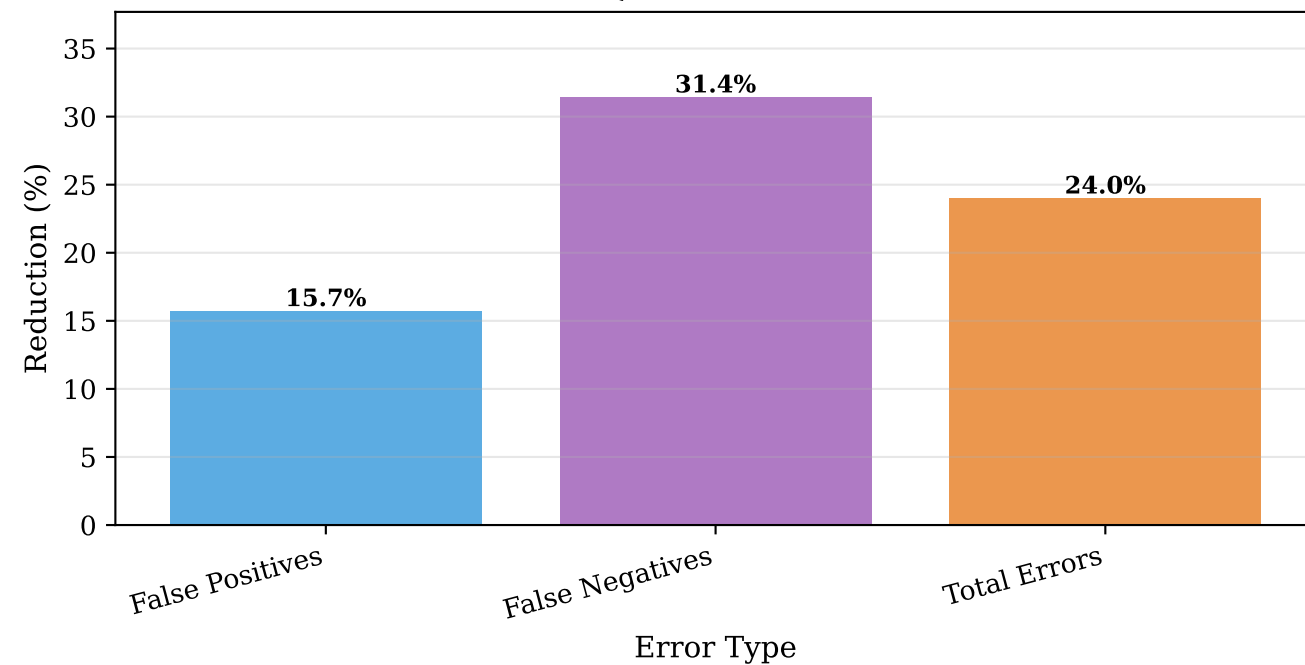
A-OKVQA: Error Reduction
