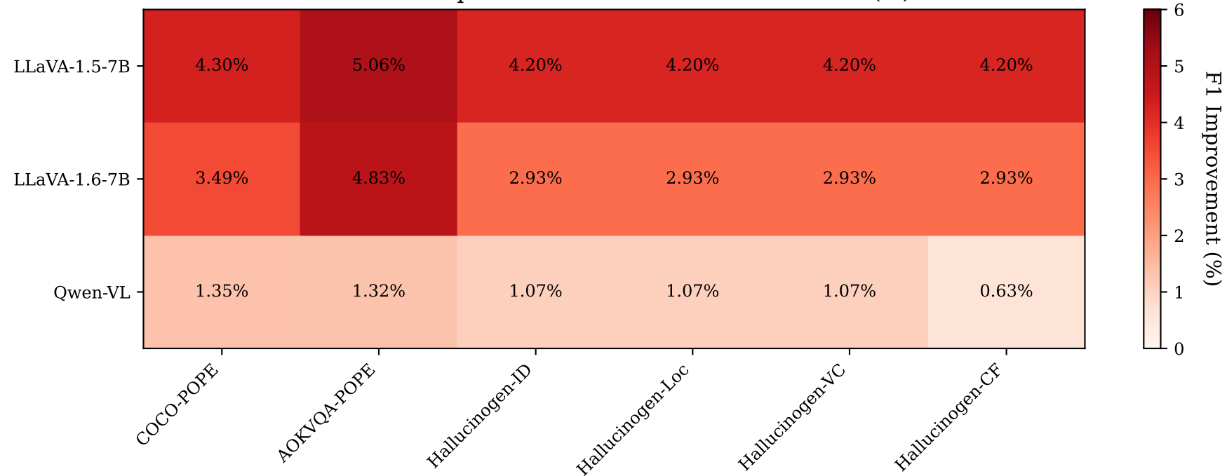
F1 Score Improvement: VCD+AGLA vs Baseline (%)
