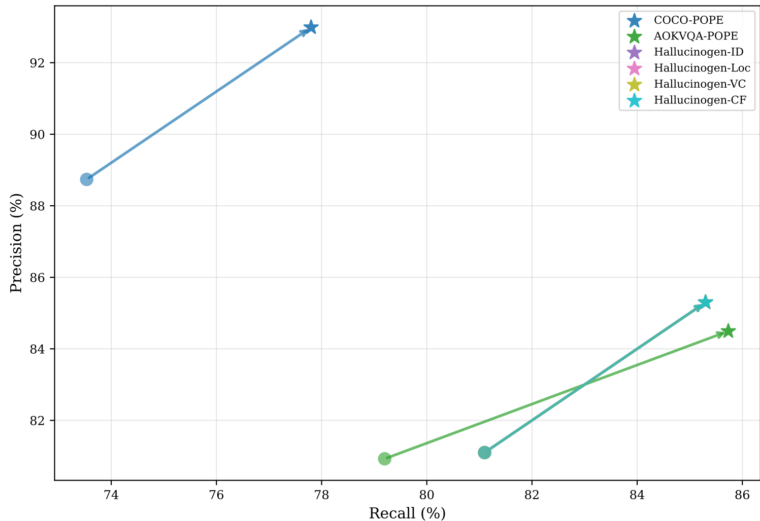
Precision-Recall Improvement: LLaVA-1.5-7B (Baseline → VCD+AGLA)
