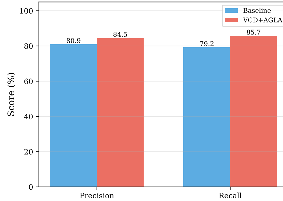
Qwen-VL COCO-POPE
