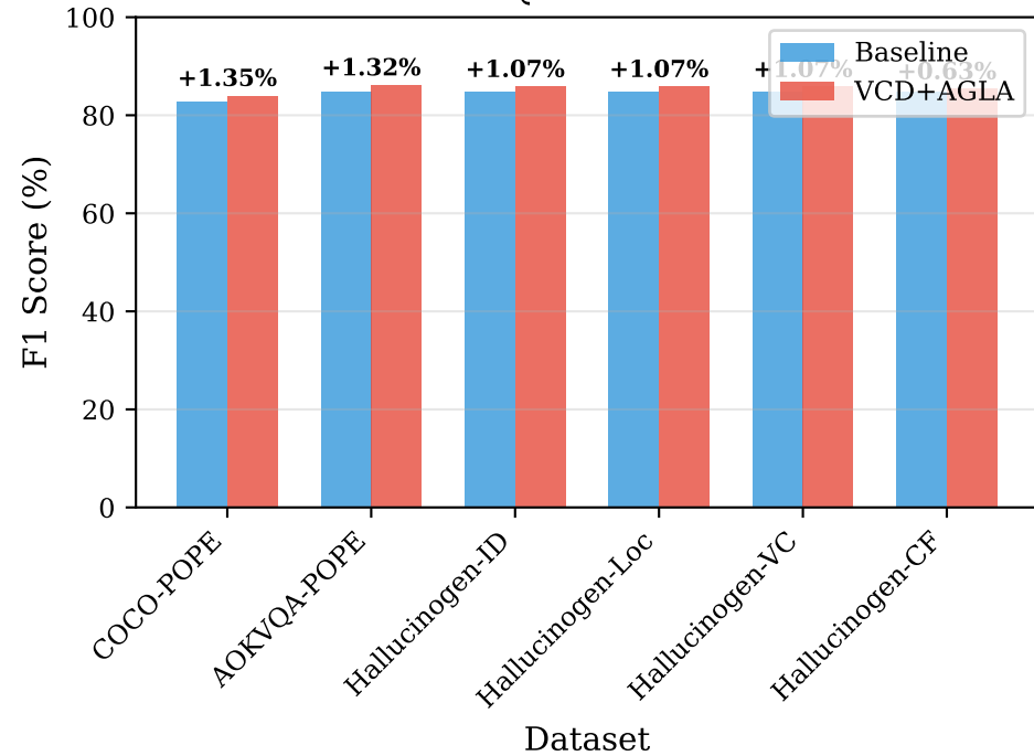
Qwen-VL
