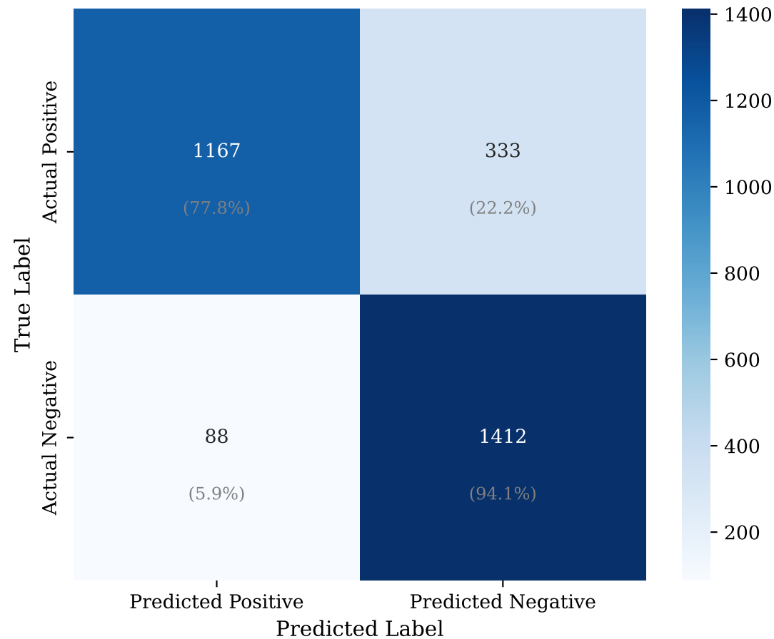
VCD+AGLA - LLaVA-1.5-7B on COCO-POPE
