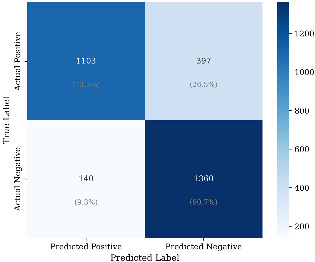
Baseline - LLaVA-1.5-7B on COCO-POPE
