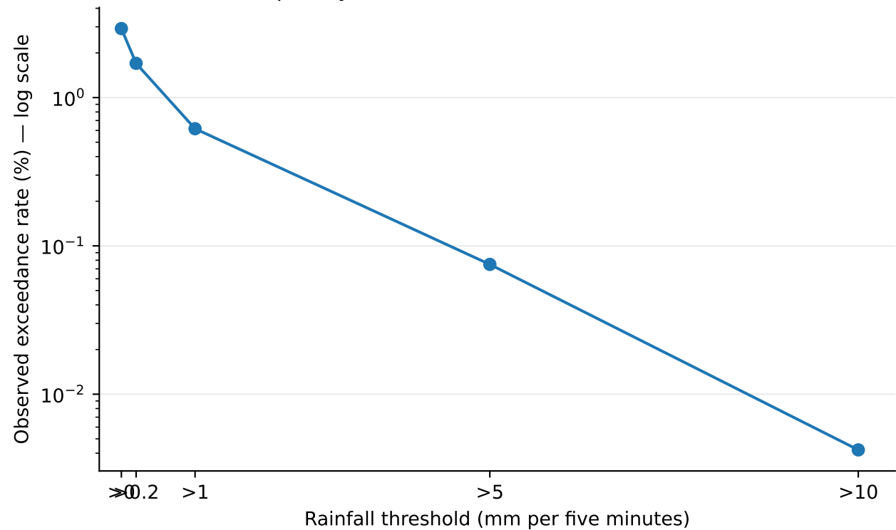
Frequency of five-minute rainfall exceedances
