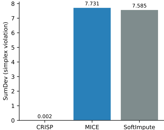
Constraint violation (lower = better)
