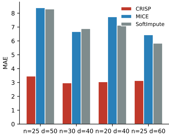
Synthetic n < d , MCAR 10%
