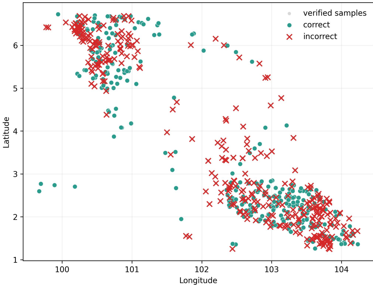
Strict spatial B3 RandomForest test errors (n=622)
