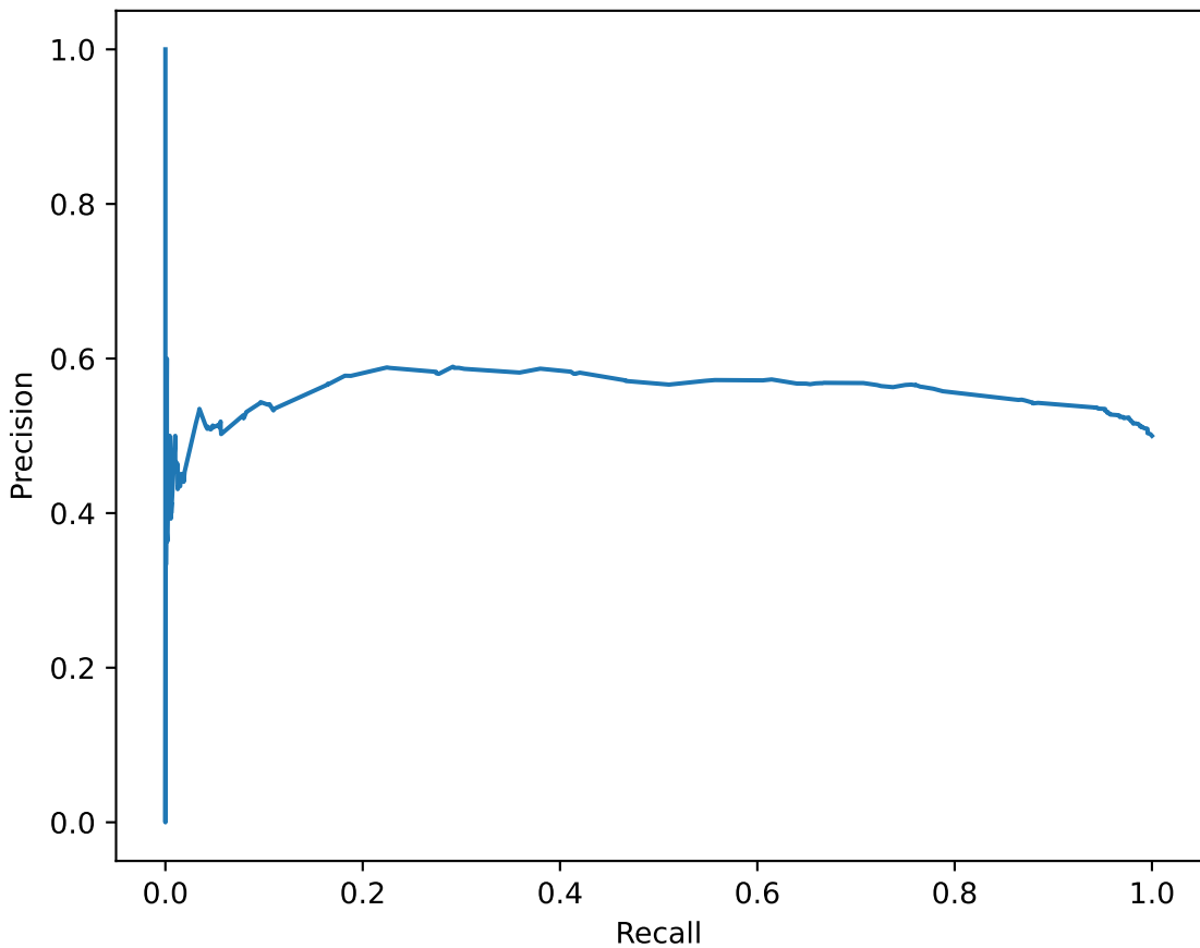
Precision-Recall
