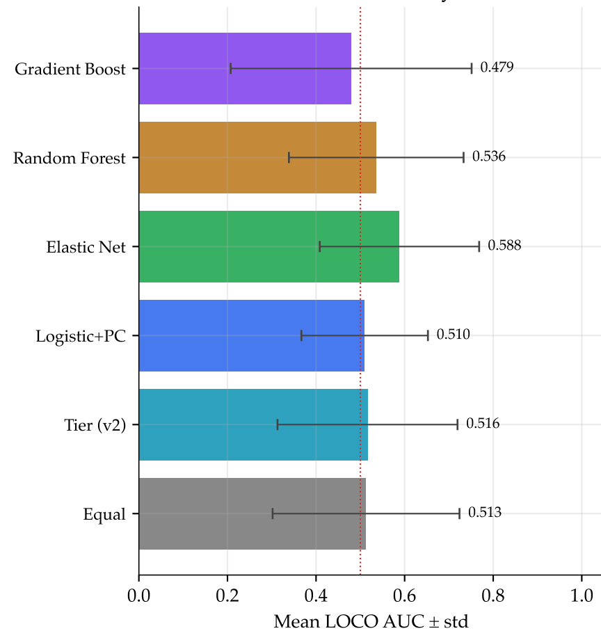
LOCO summary
