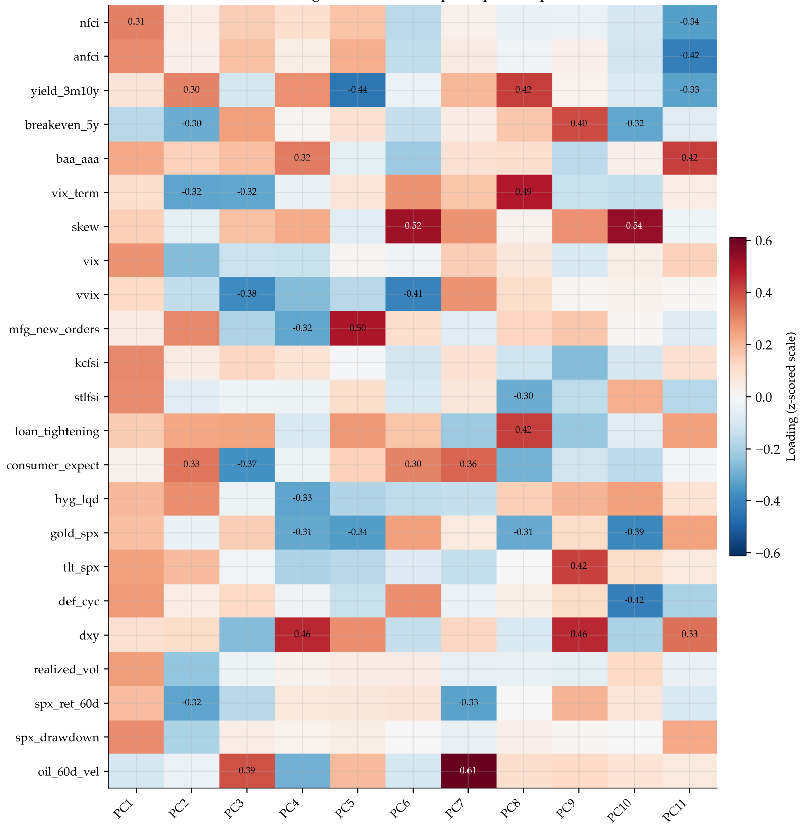
PCA loadings — indicators × principal components
