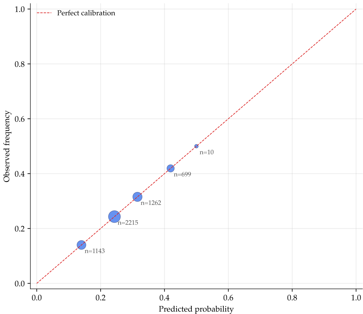
Reliability diagram — equal_weight + isotonic Brier 0.1856 (baseline 0.1932)
