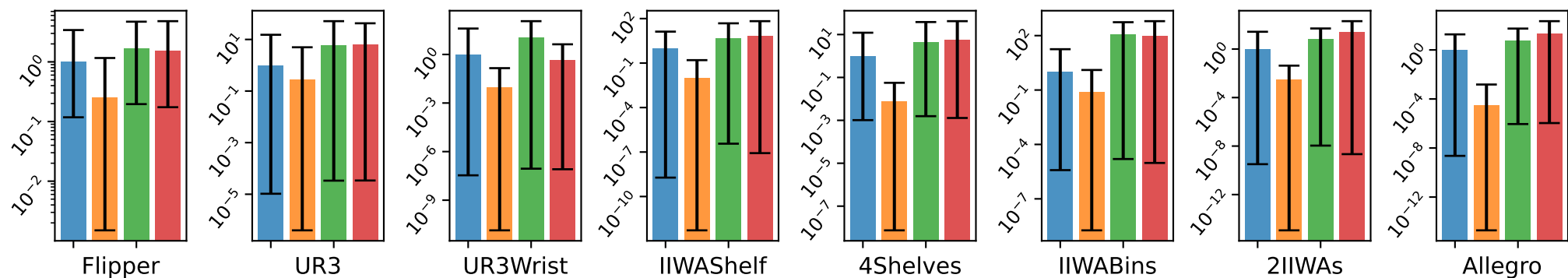
fraction_in_collision
