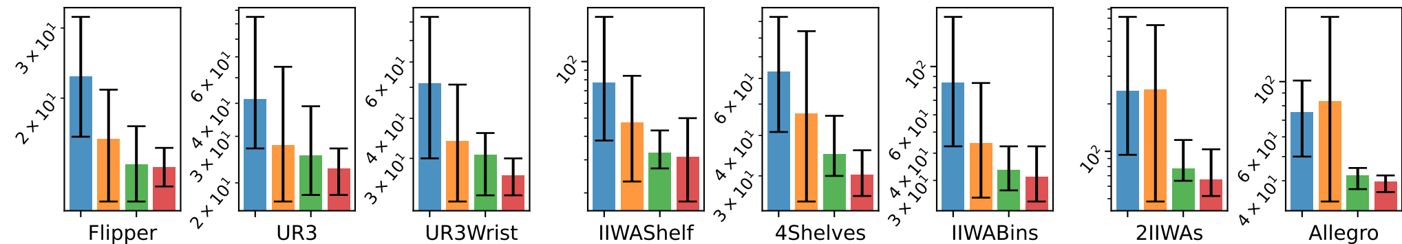
num_faces
