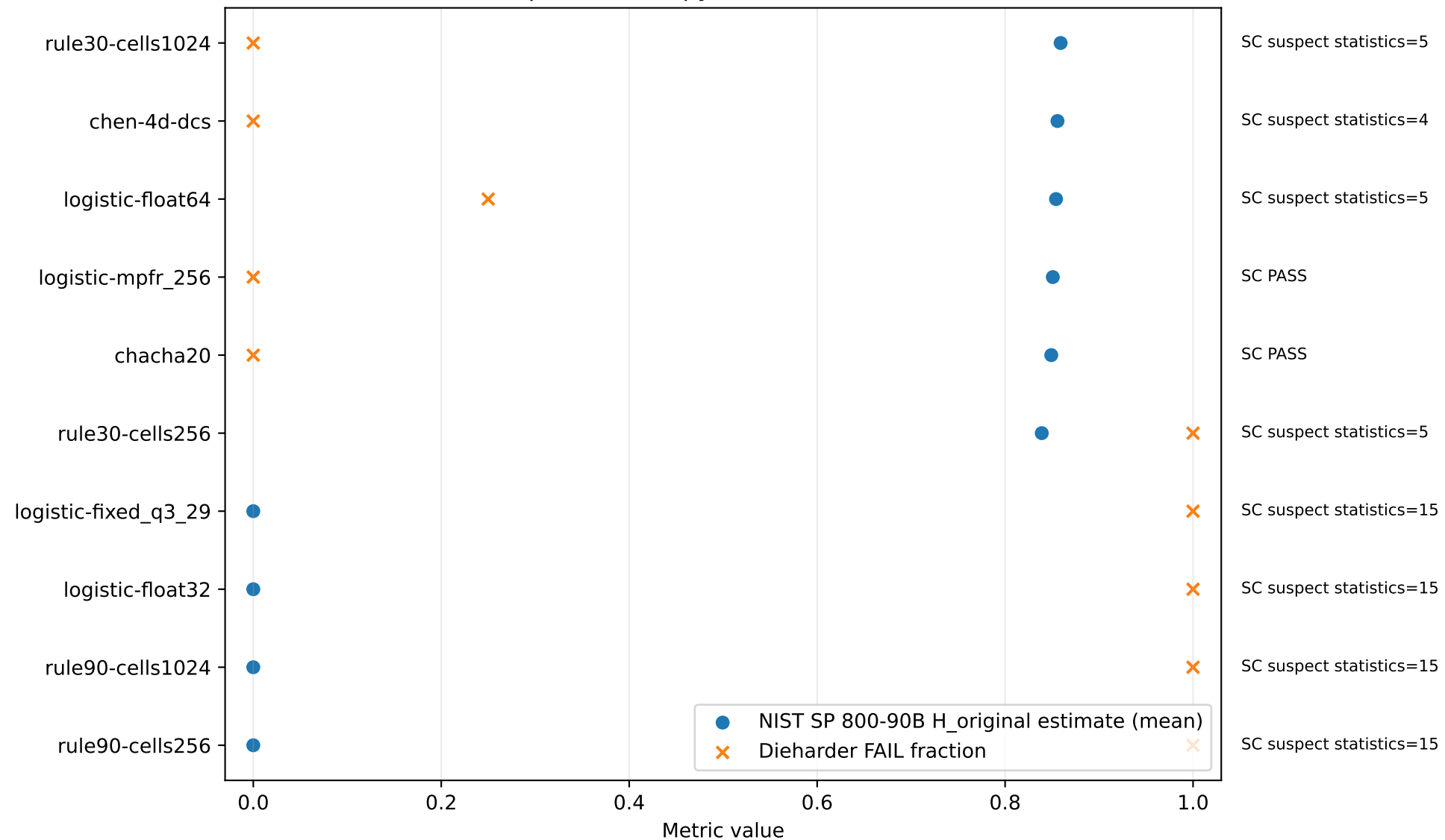
Frozen local source profile: entropy estimate, Dieharder and SmallCrush
