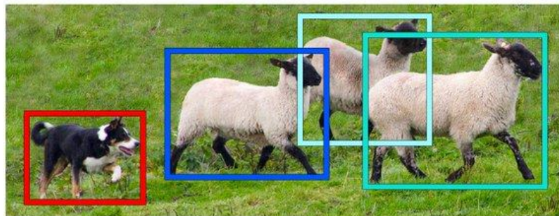
Object Detection
