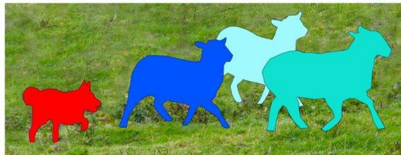
Instance Segmentation
