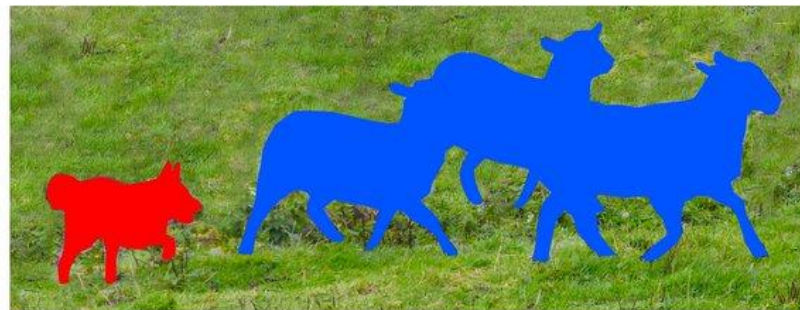
Semantic Segmentation
