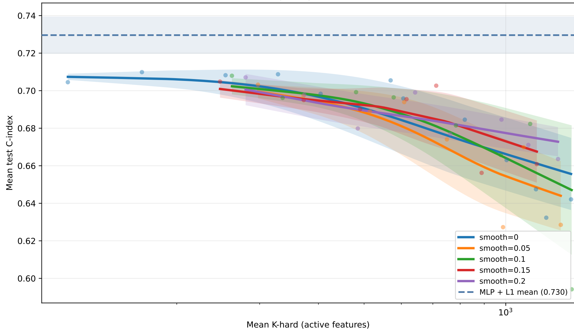
Concrete C-index vs sparsity — with MLP+L1 reference
