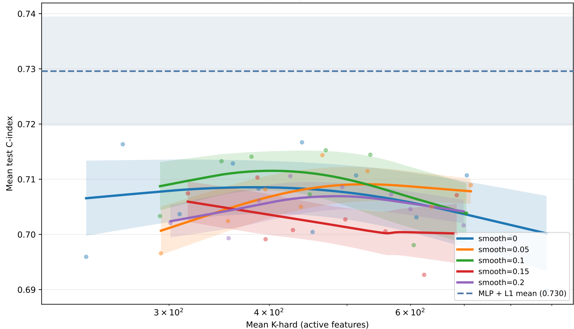
LSPIN C-index vs sparsity — with MLP+L1 reference
