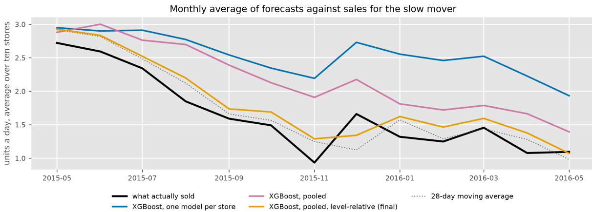
Figure 5. Why the first model lost on the slow mover. Sales fell through the year and the per-store trees stayed near the old level. The final model tracks the decline alongside the moving average.
