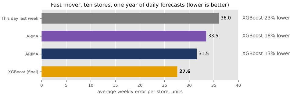
Figure 1. The fast mover's average weekly error per store over the test year. The final model is gradient-boosted trees (XGBoost) trained across all ten stores on a level-relative target. ARMA has no seasonality and no holiday or SNAP inputs. ARIMA is seasonal, with those inputs, and is the strongest statistical model here.
