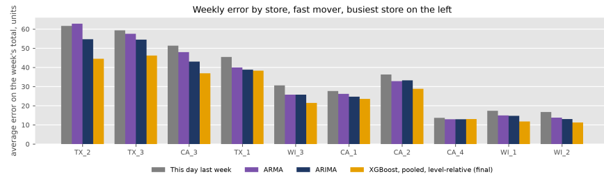
Figure 2. Average weekly error by store, in units, busiest on the left. The final model's error is lower than last week's number at every store and lower than ARMA's and ARIMA's at nine of ten, level at the tenth. The busiest store benefits the most, 17 fewer units a week.
