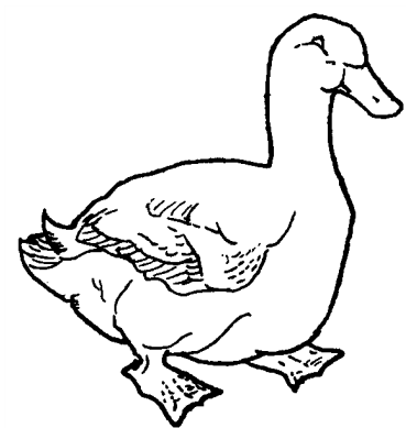
Figure 7.1: Cohen's duck
