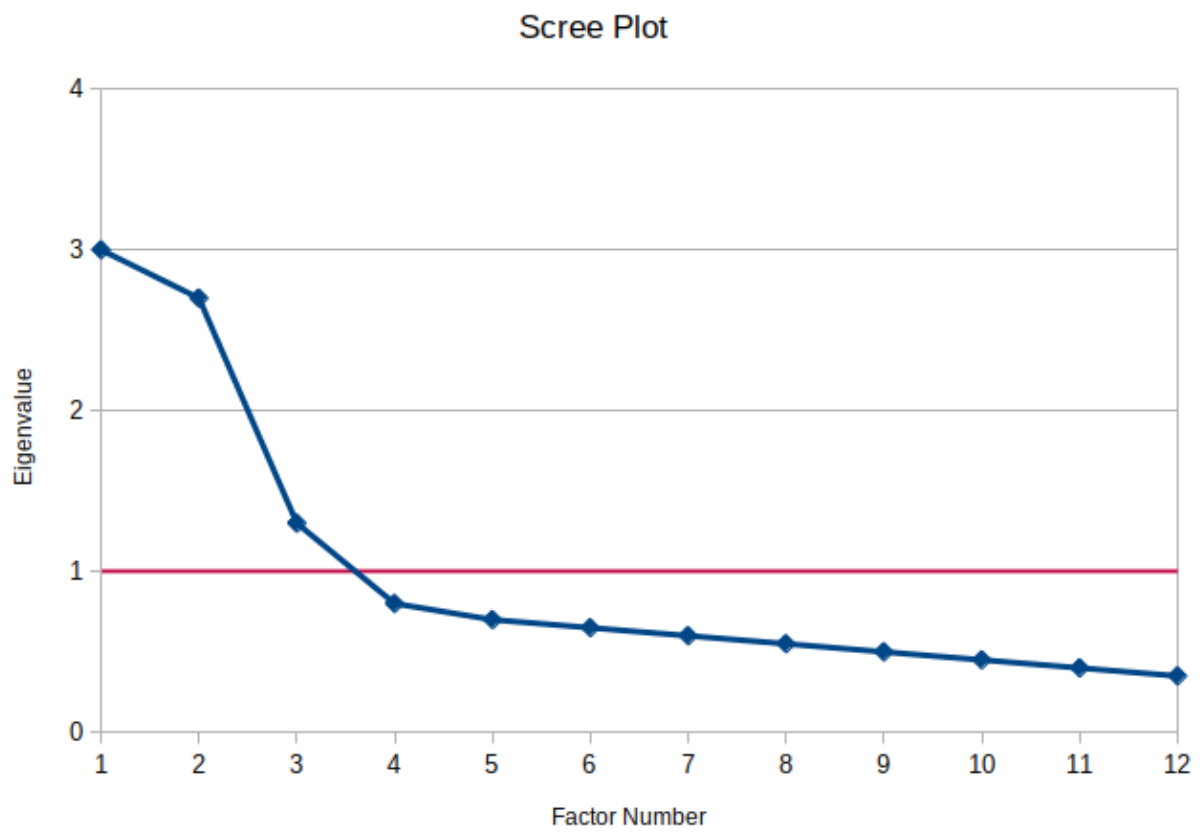
Figure 13.1: Example Scree Plot of a 12-Item Instrument
