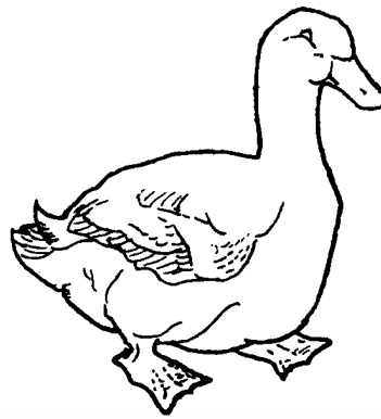
Figure 6.1: Cohen's duck
