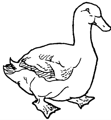
Figure 6.1: Cohen's duck
