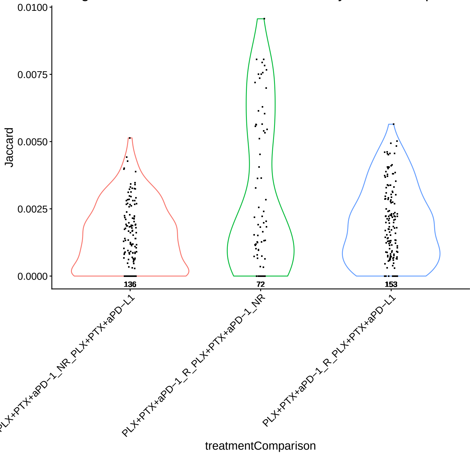
Fig S7a – Jaccard Index Between Primary Tumor Samples
