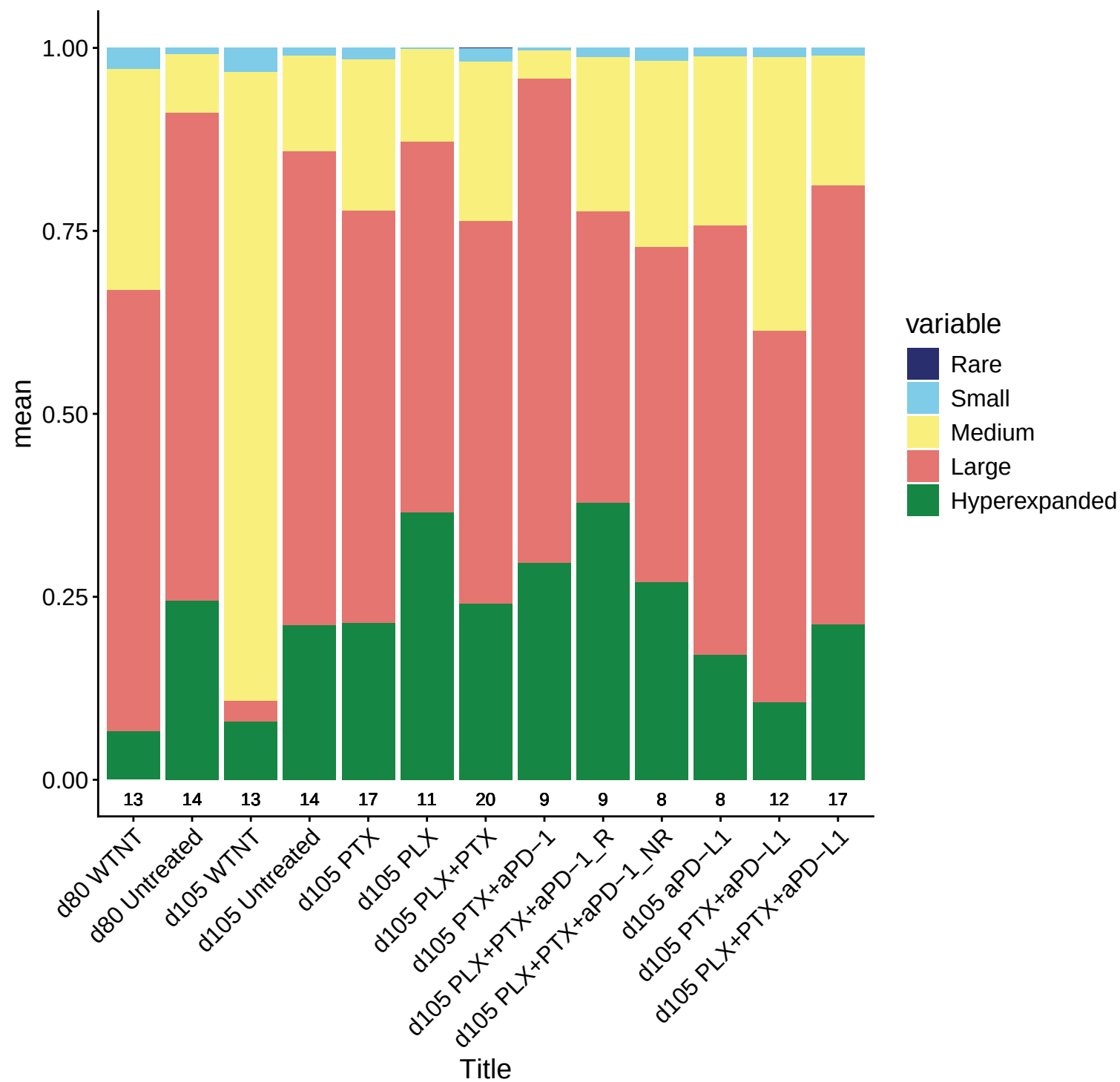
Fig 7d – Binned Clonal Frequencies of Primary Tumors
