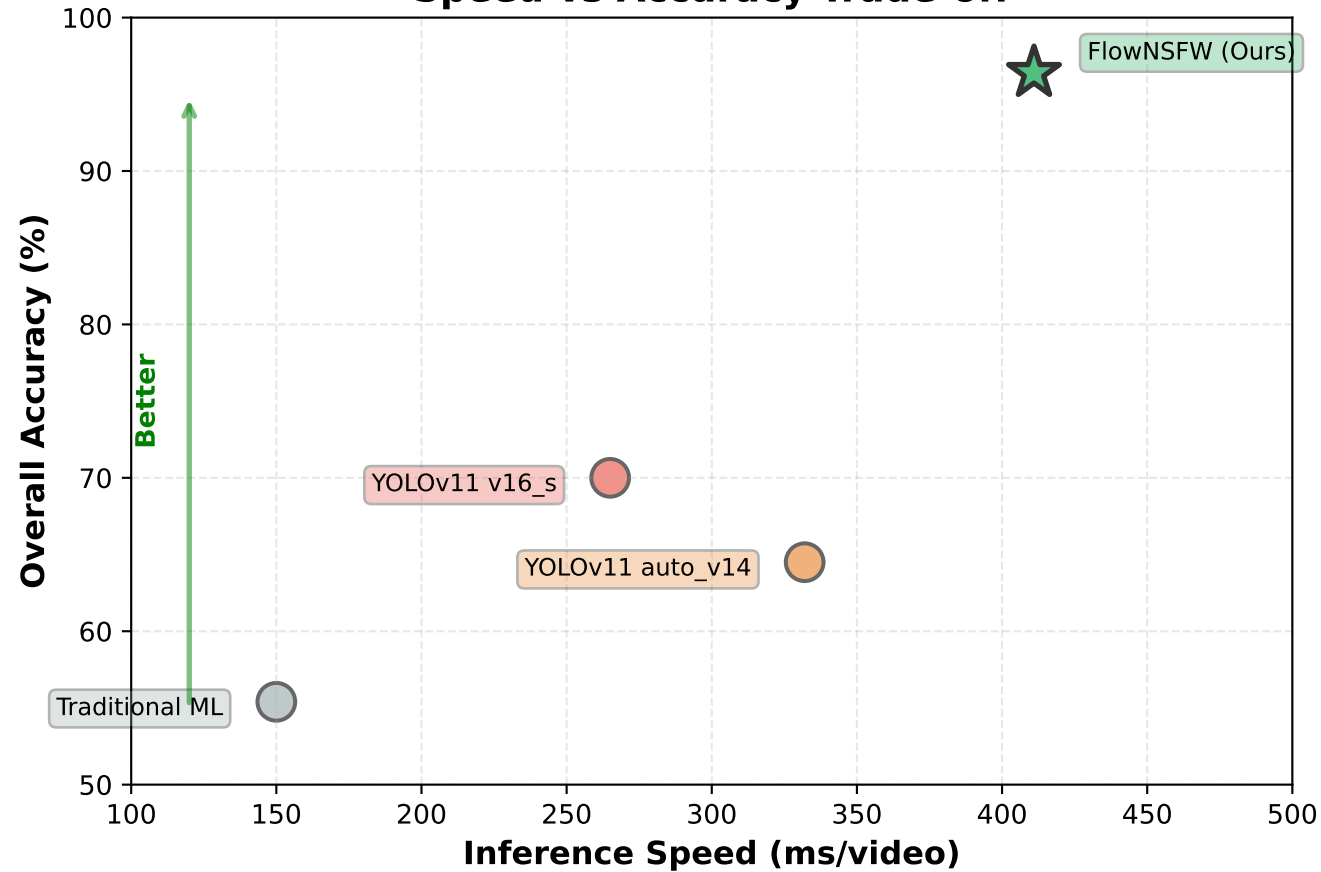
Speed vs Accuracy Trade-off
