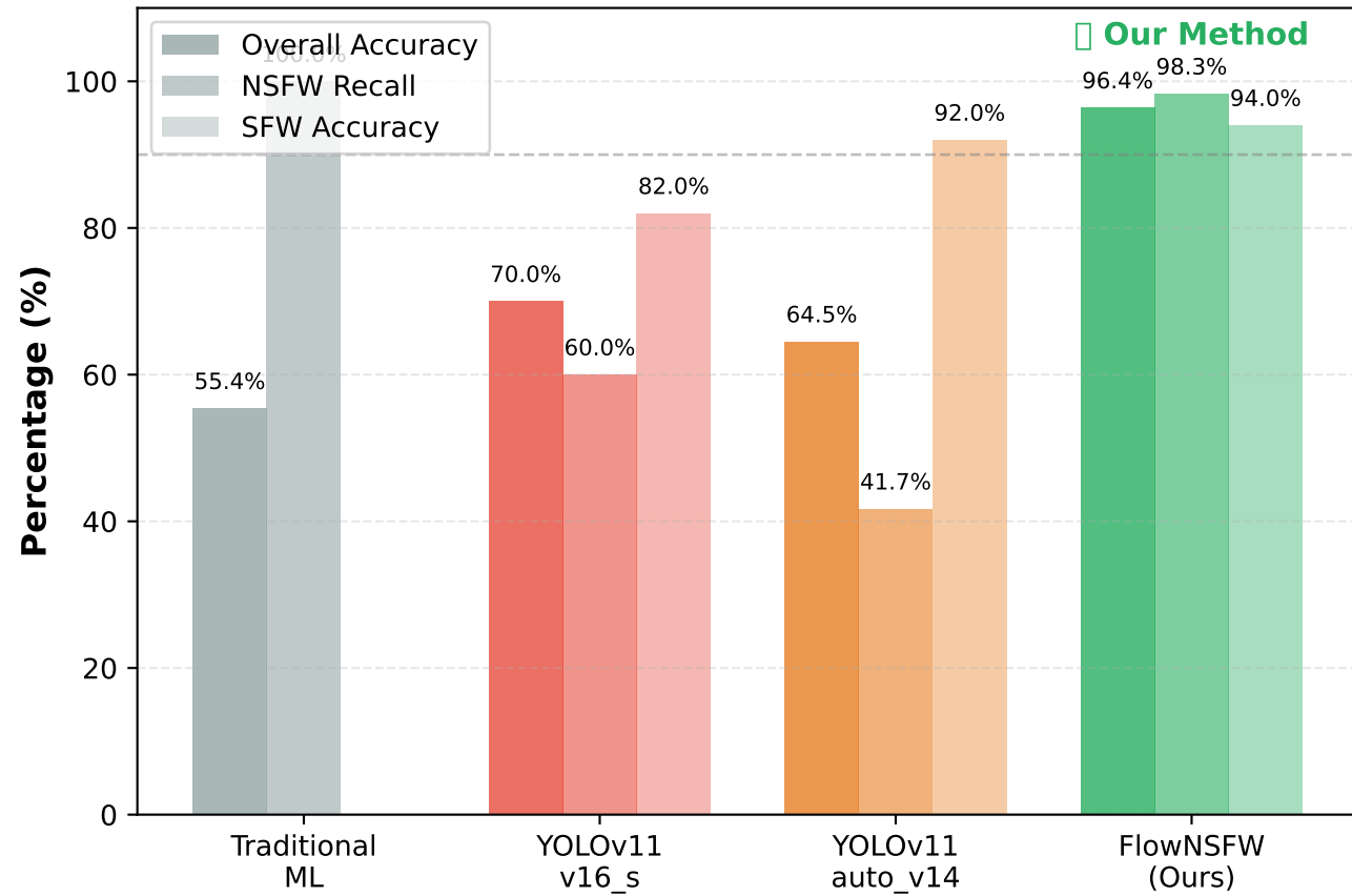
Performance Comparison (224 Test Videos)
