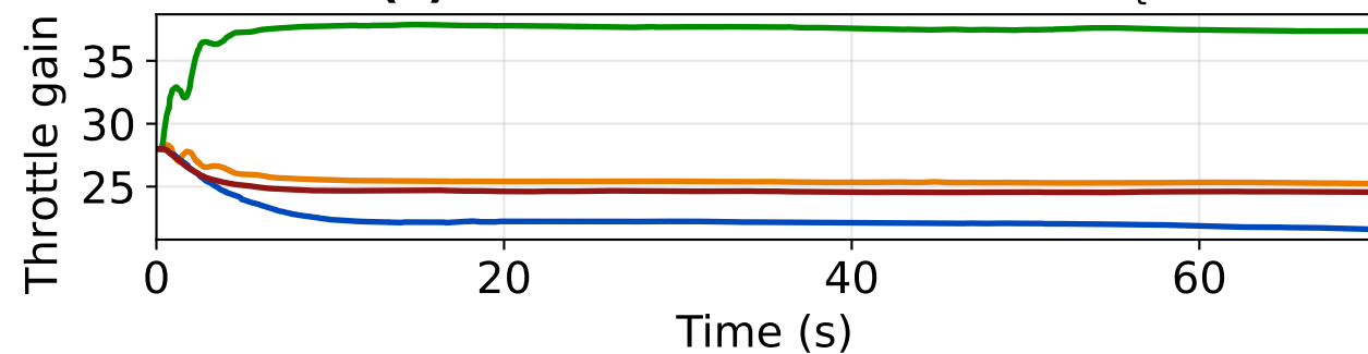
(c) Estimated Throttle Gain \hat{k}_t
