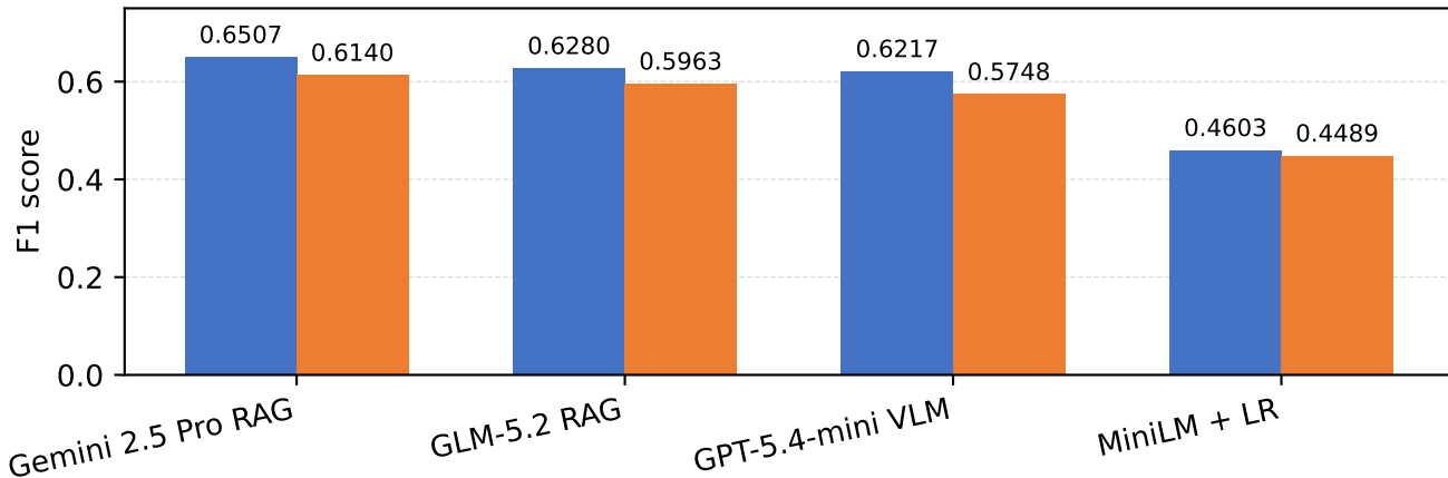
Task 2 Single-Page Metric Verification: Micro F1 and Macro F1 by Model
