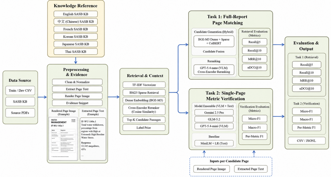
Figure 1: Generated unified architecture for Task 1 full-report page matching and Task 2 single-page metric verification. The diagram shows the shared multilingual knowledge and evidence path, Task 1’s BGE-M3 retrieval and VLM reranking branch, Task 2’s page-image verification models, and the corresponding evaluation outputs.
