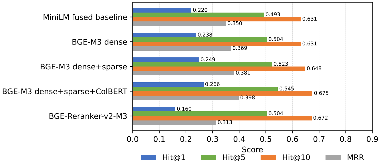
Task 1 retrieval comparison (369 non-empty-gold groups)
