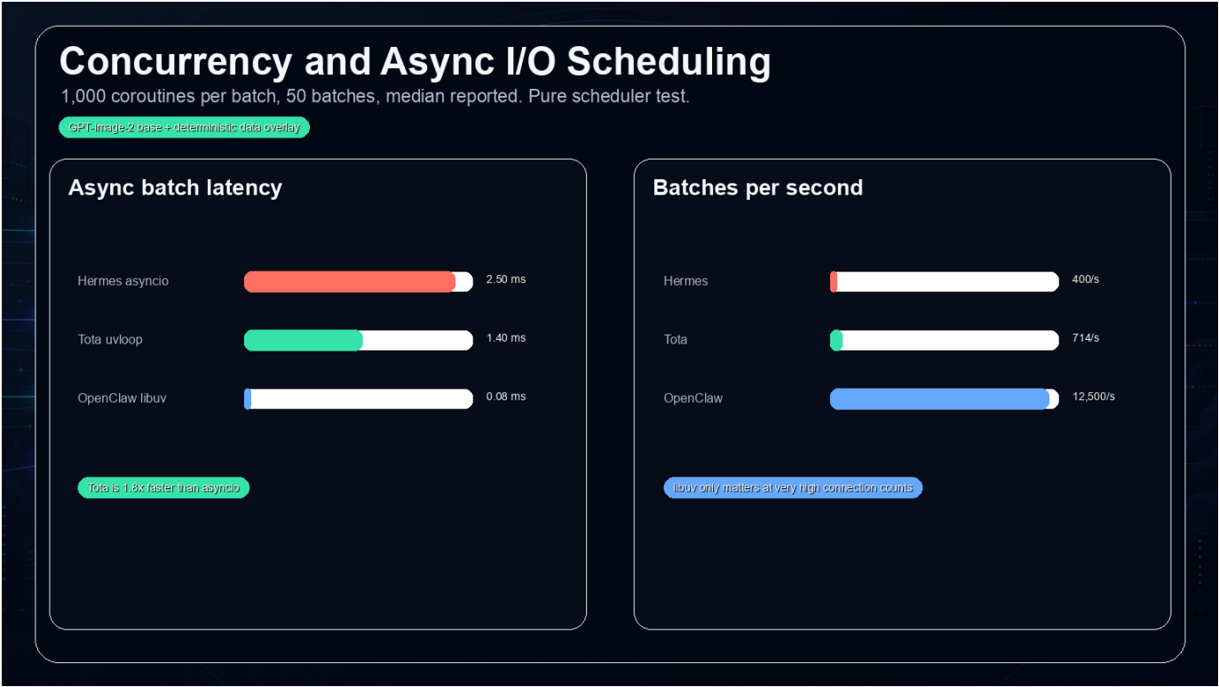
Figure 6 - Concurrency and async scheduling.
