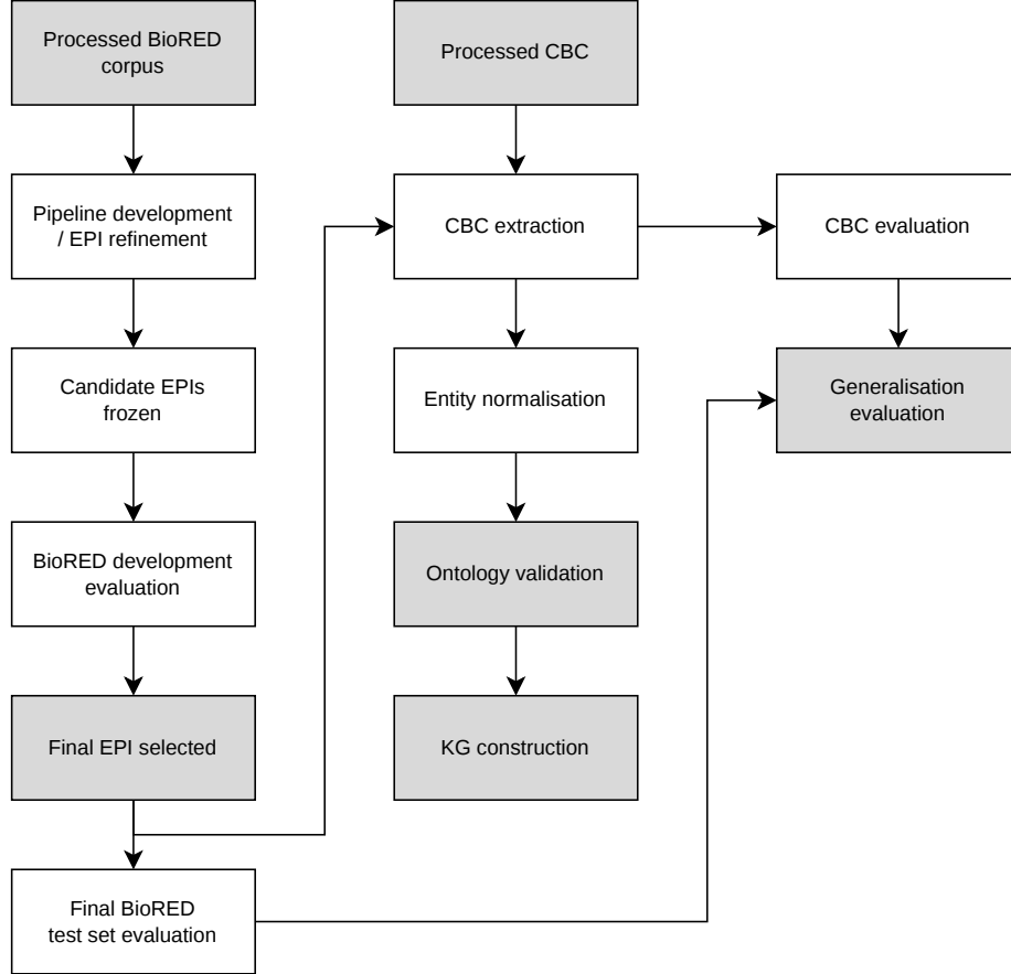
Figure 4.1: System architecture and data flow, from prepared corpus input through extraction, normalisation, and KG construction, to the three evaluation branches described in Section 4.7. Grey shading highlights key inputs, final stages, and outputs.
