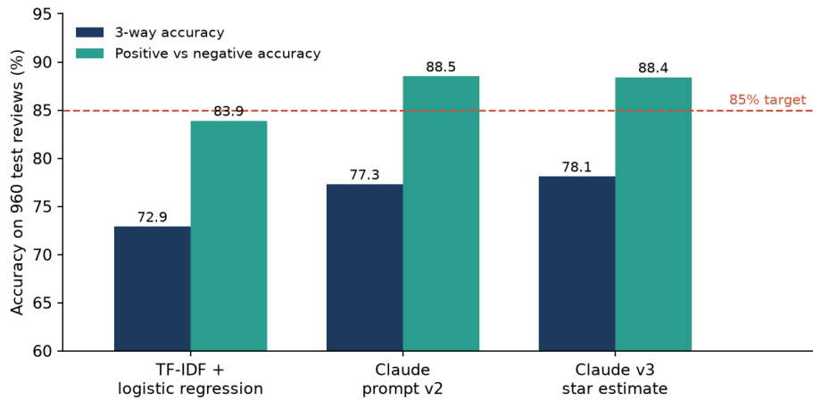
Figure 2. Sentiment accuracy on the 960 held-out test reviews.
