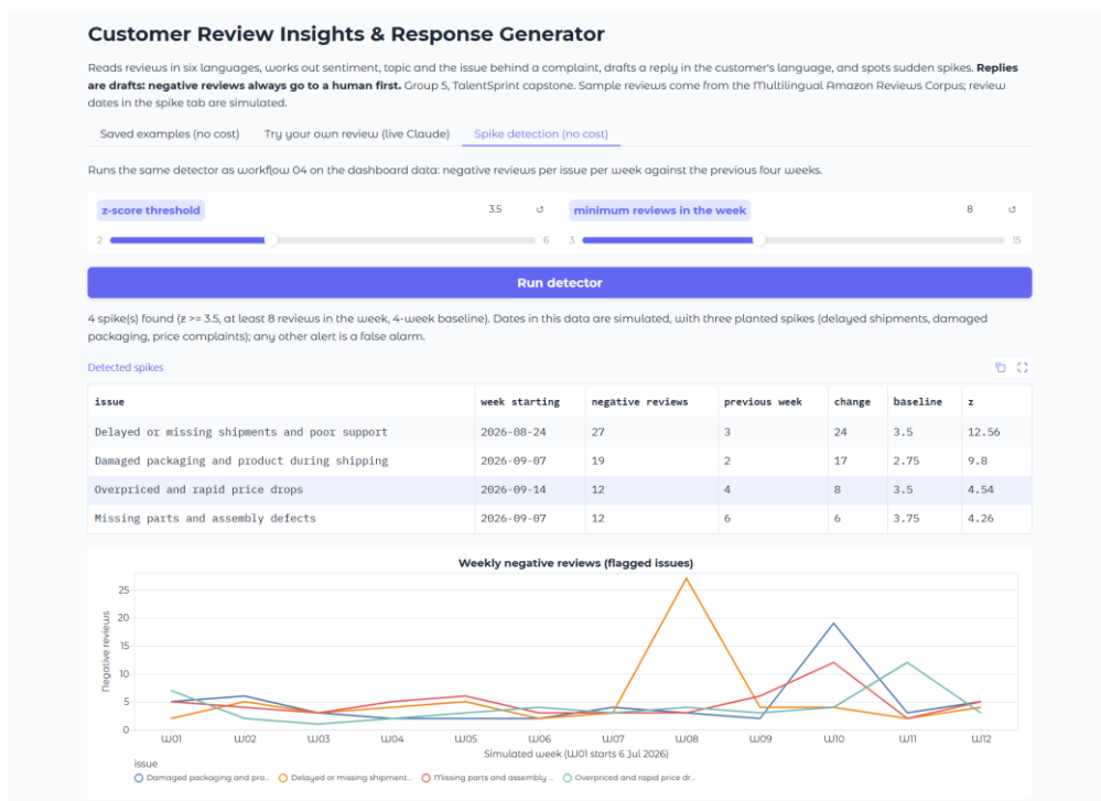
Figure B6. Demo app, "Spike detection" tab: the four spikes (z-score 12.56, 9.80, 4.54 and 4.26) and the weekly line chart; the same detector as workflow 04.
