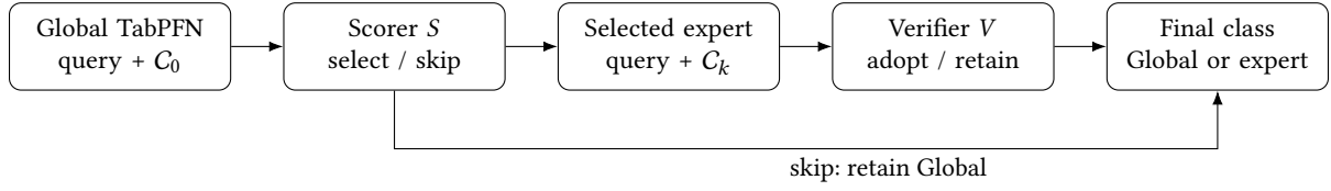
Figure 1: Query-time decisions in the current design. The context bank is constructed beforehand from training data. A scorer selects at most one expert; a verifier may retain the Global output even after that expert is called. The current experiments evaluate this policy using cached expert predictions, not a measured online conditional-inference service.
