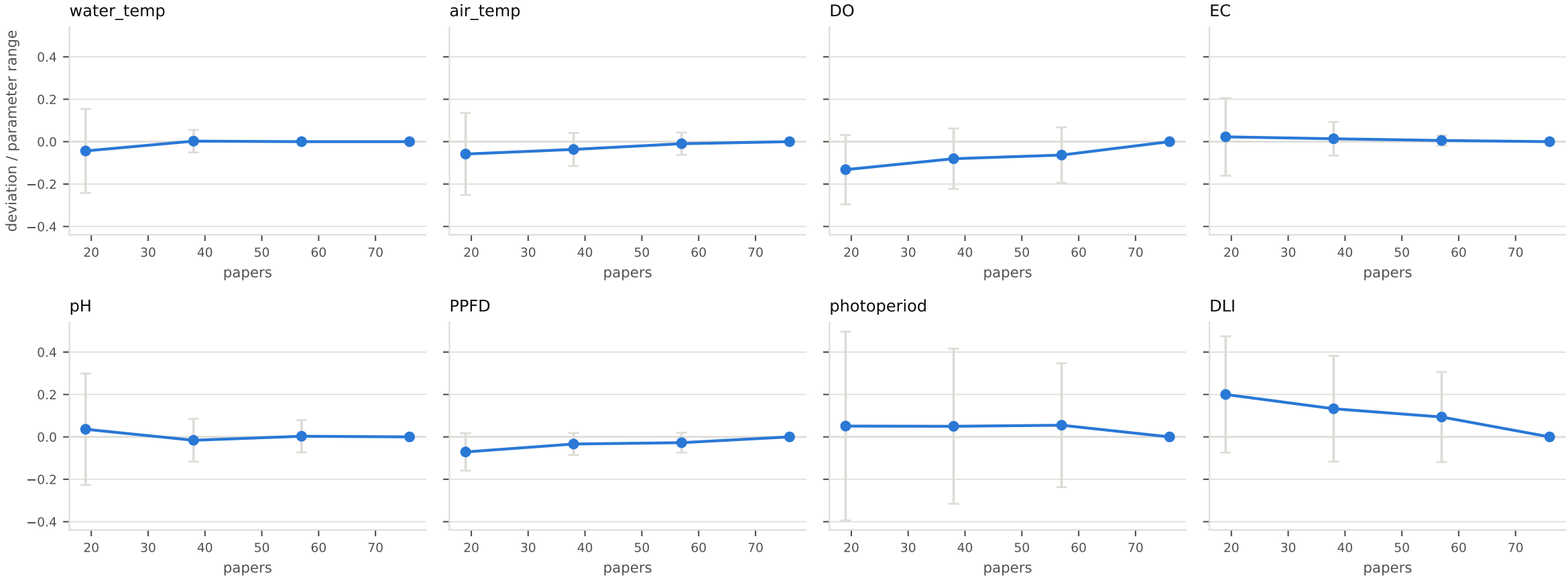
Convergence to the full-corpus value (100 draws per size); bars = s.d. across draws
