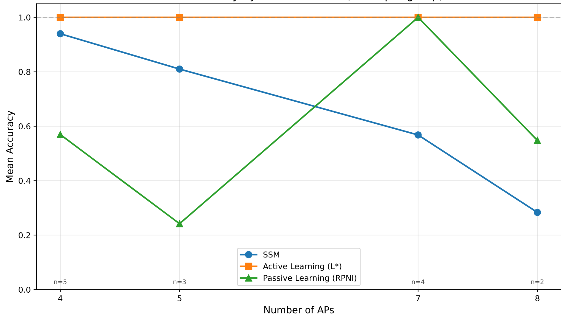
Mean Accuracy by Number of APs ( n \geq 2 per group)
