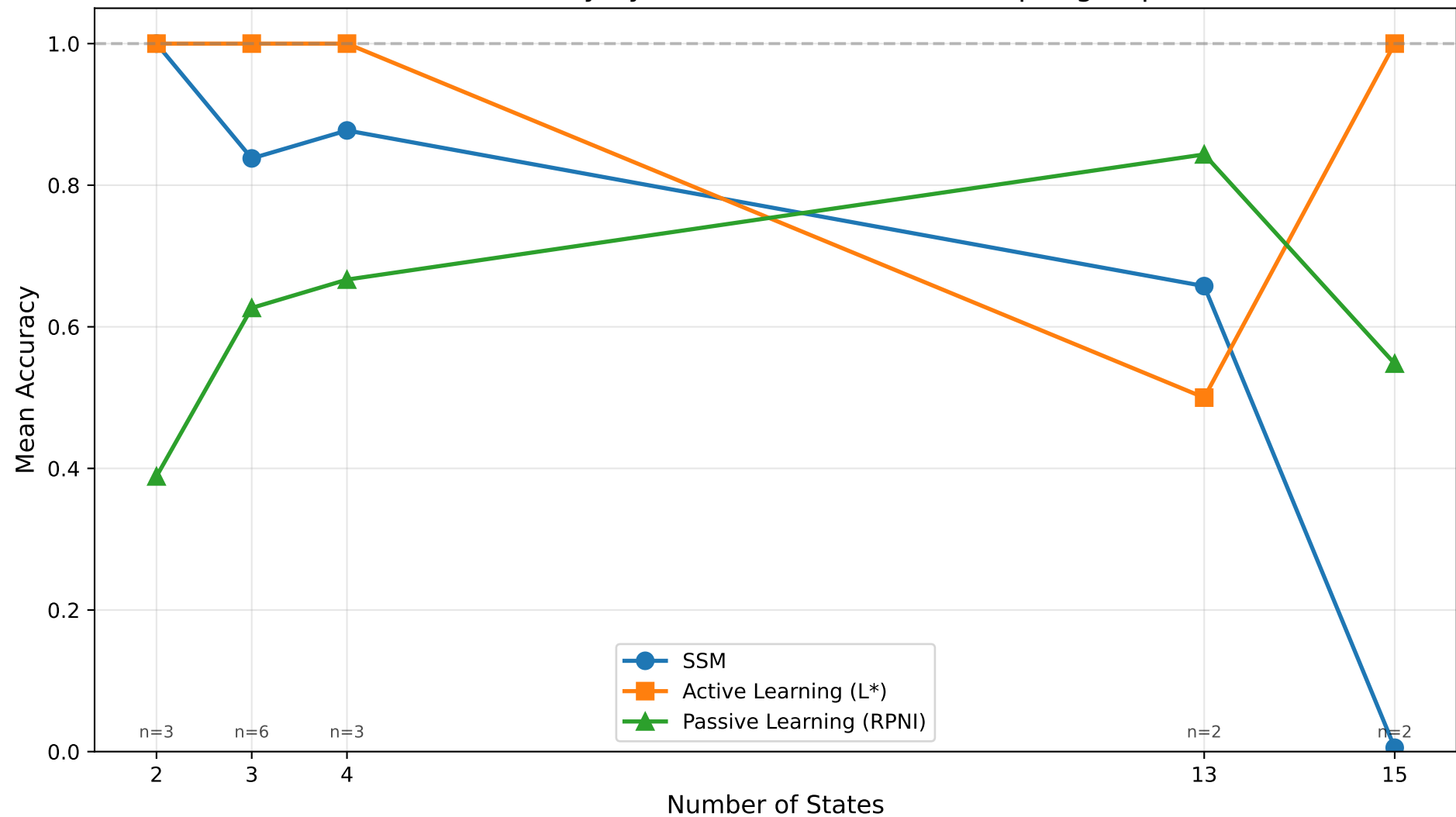
Mean Accuracy by Number of States ( n \geq 2 per group)
