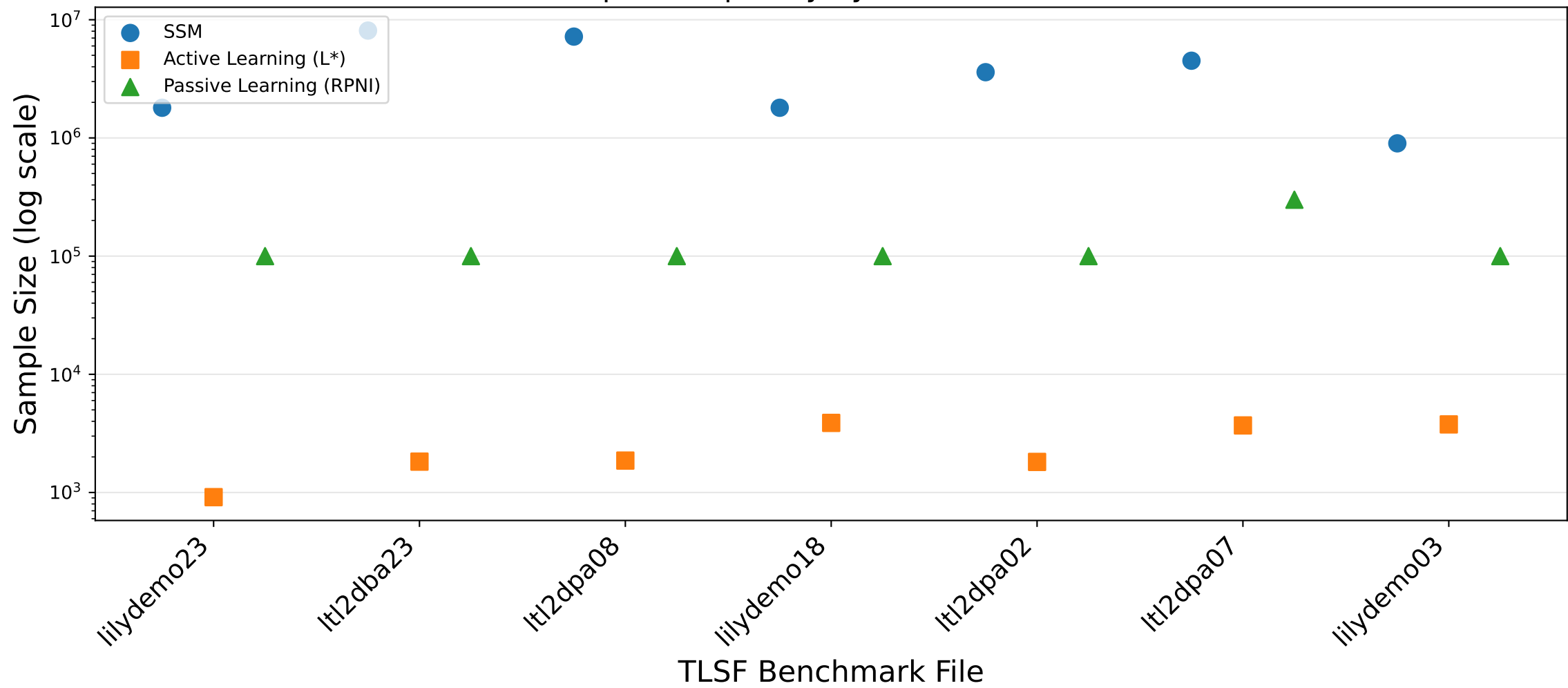
Sample Complexity by TLSF Benchmark
