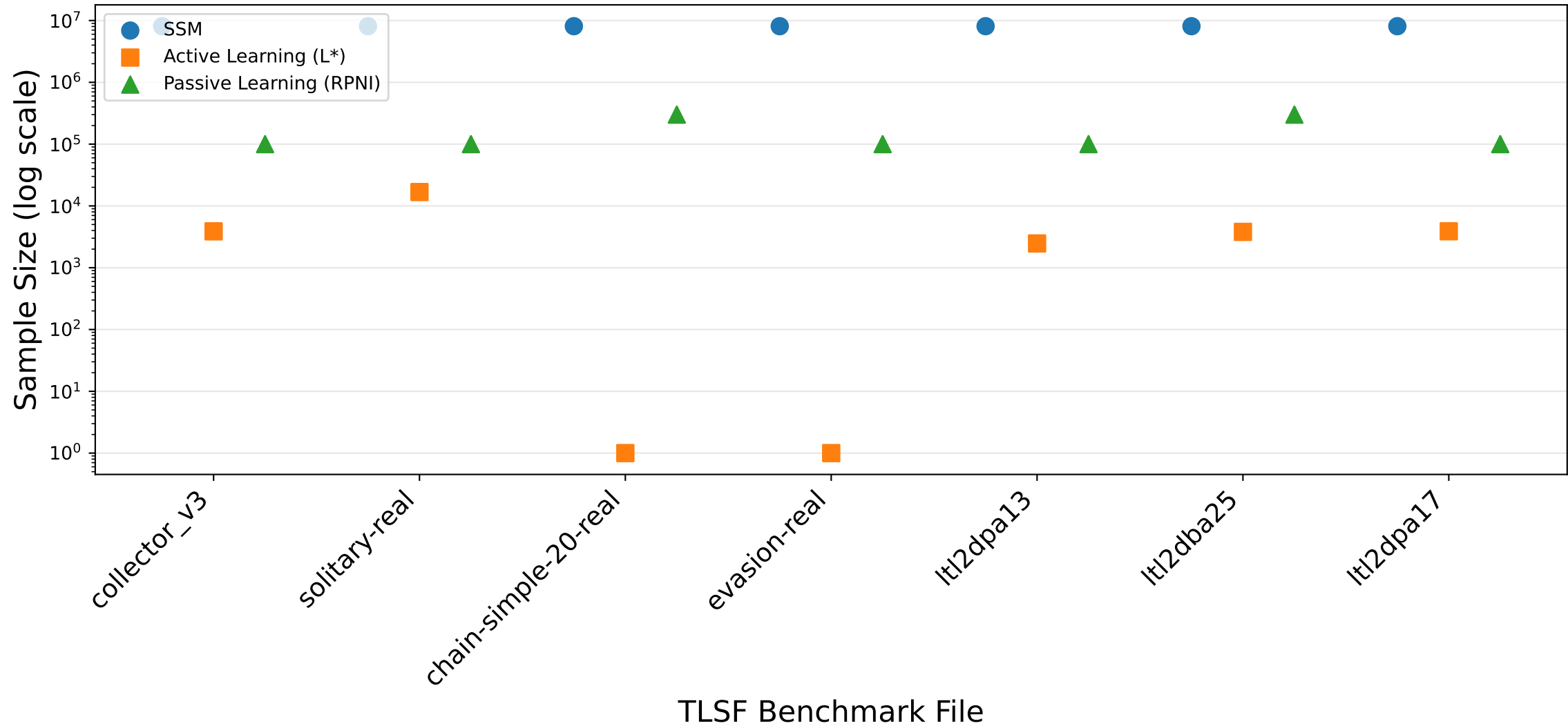
Sample Complexity by TLSF Benchmark
