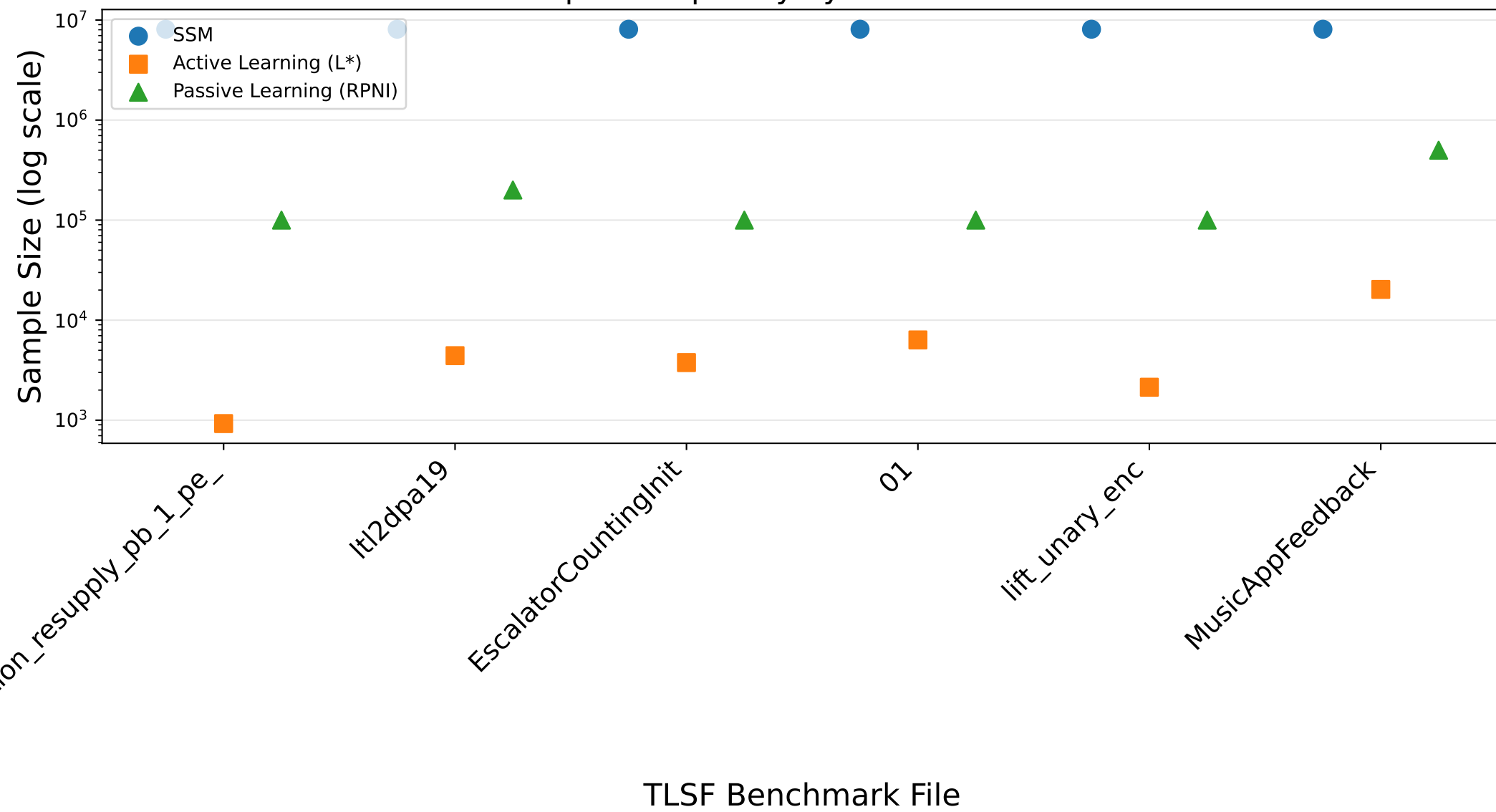
Sample Complexity by TLSF Benchmark
