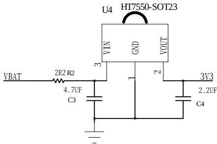
LD03V3
