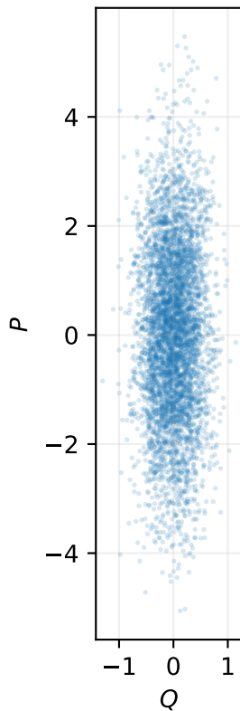
Squeezed-vacuum Wigner samples ( r = 0.8 )
