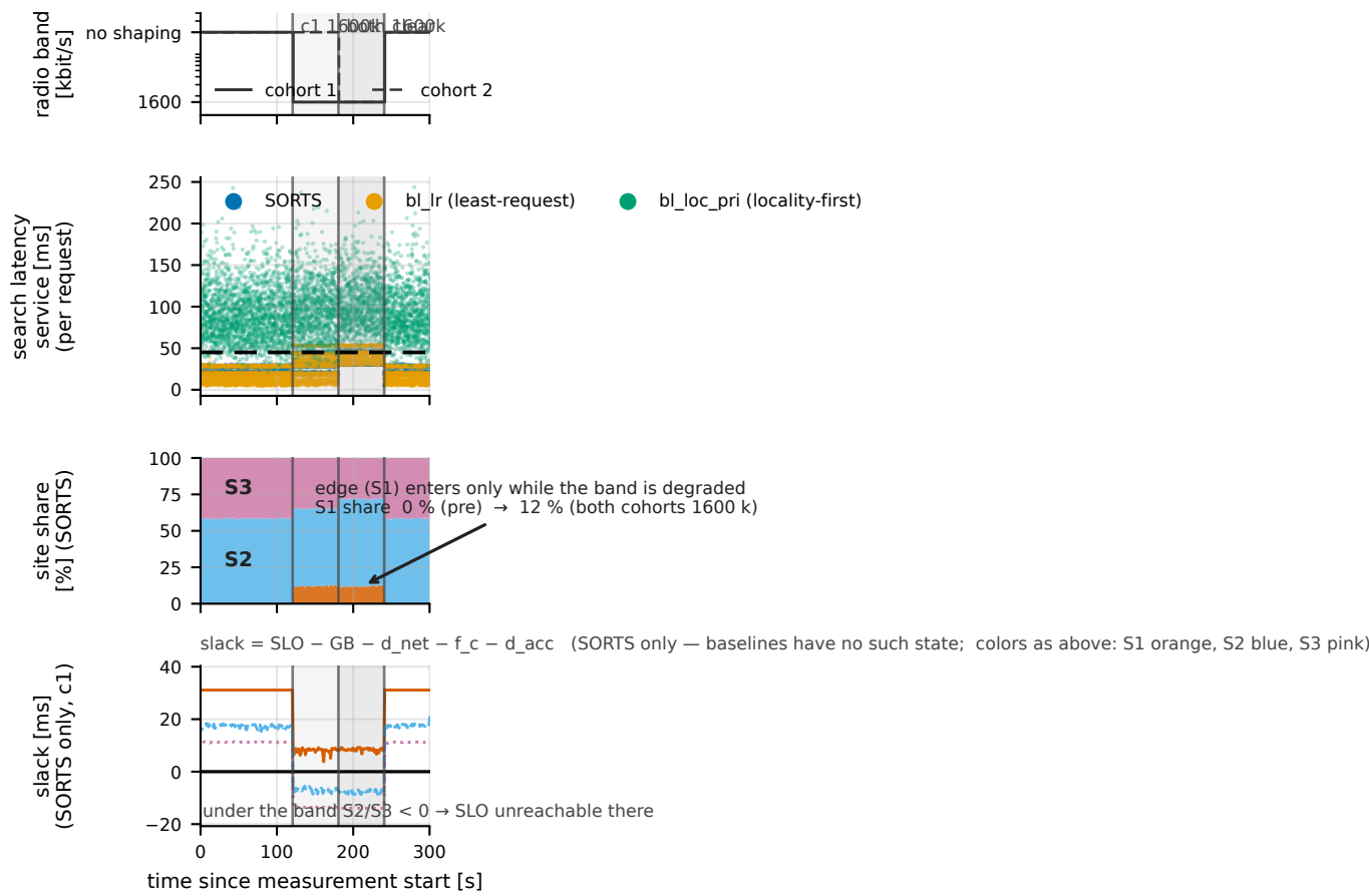
F1 Radio degradation → routing response (L = 800 rps, seq_extreme 1600 kbit, 2 cohorts, hc_off)
